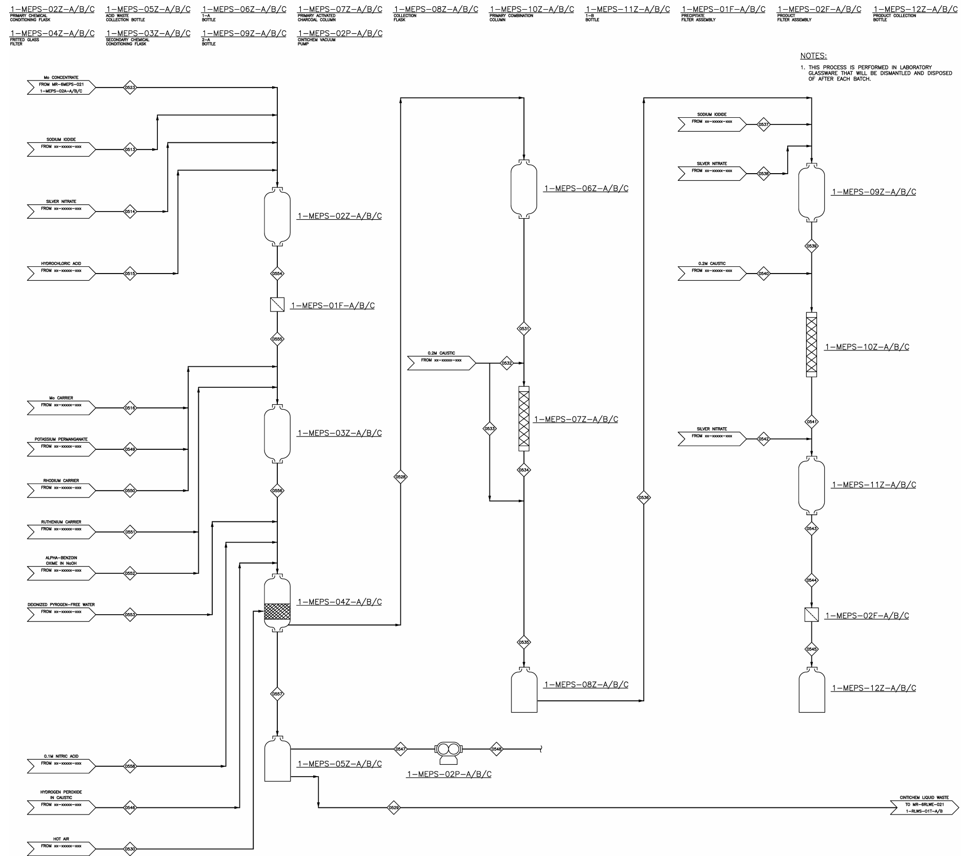
Figure 4b.3-2 – Purification Process Flow Diagram
