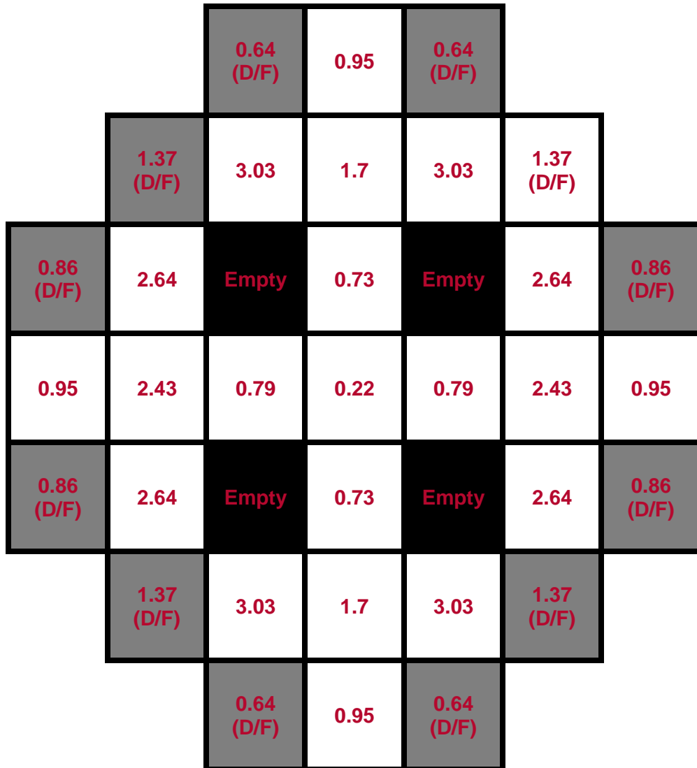
Figure 2.3-14: Loading Pattern 1 for MPC-37P
