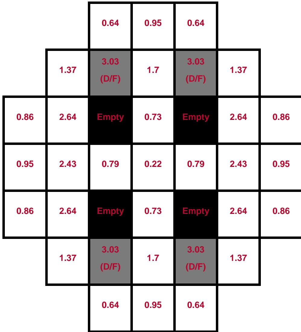
Figure 2.3-15: Loading Pattern 2 for MPC-37P
