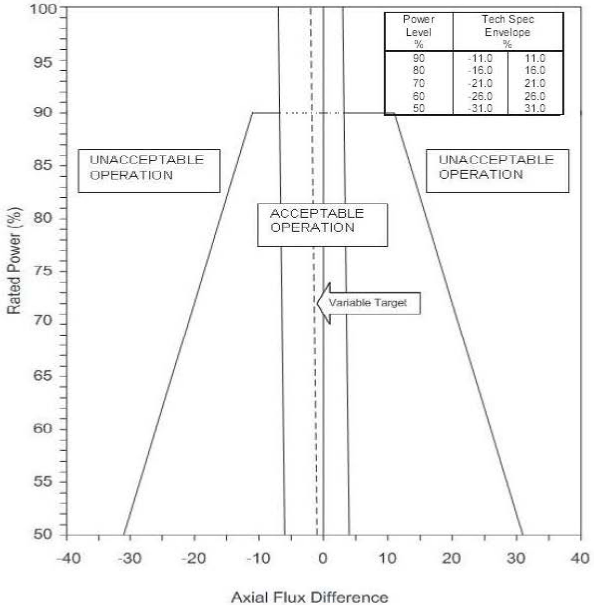
FIGURE 8 FLUX DIFFERENCE OPERATING ENVELOPE
