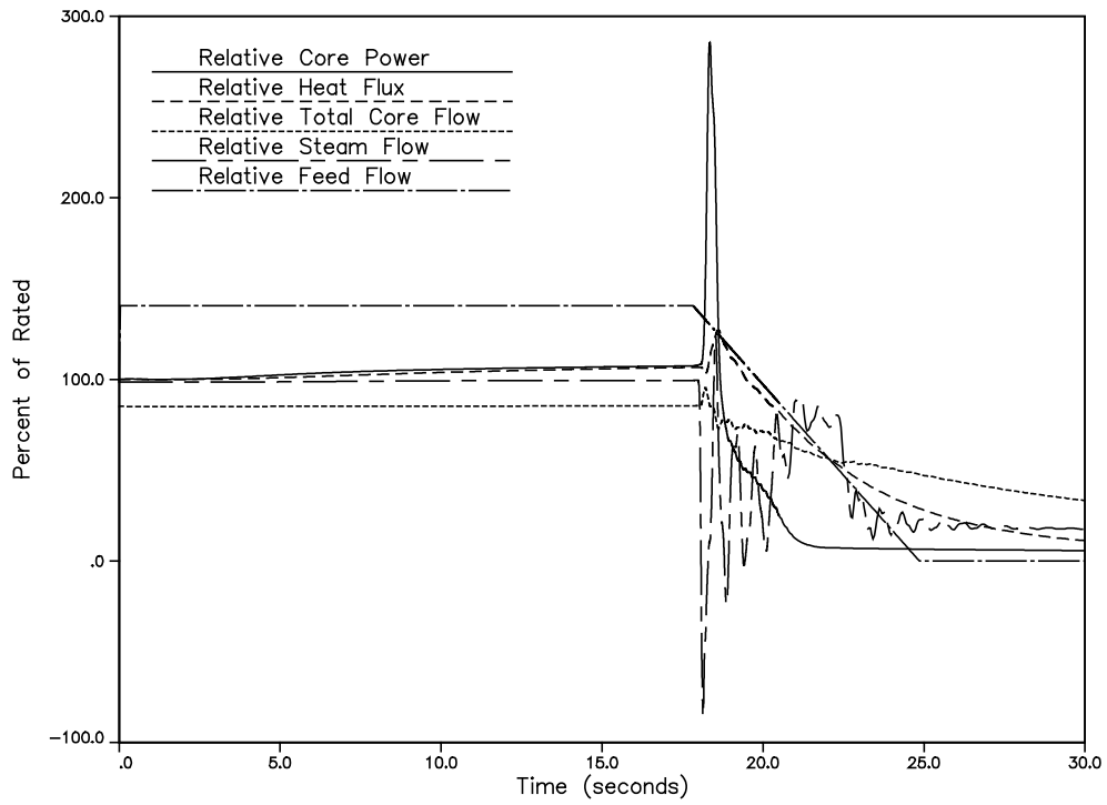
Figure 4 EOCLB FWCF at 100P/85F – TSSS Key Parameters
