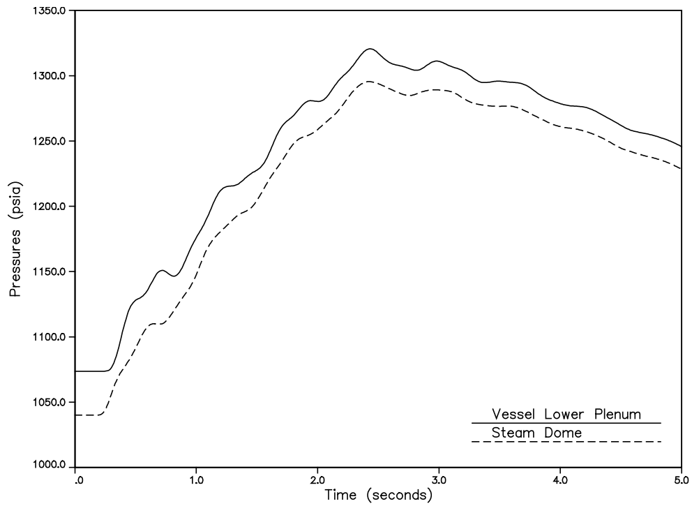
Figure 3 EOCLB LRNB at 100P/85F – TSSS Vessel Pressures
