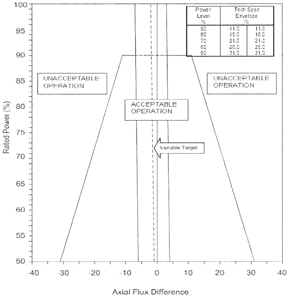
FIGURE 6 FLUX DIFFERENCE OPERATING ENVELOPE
