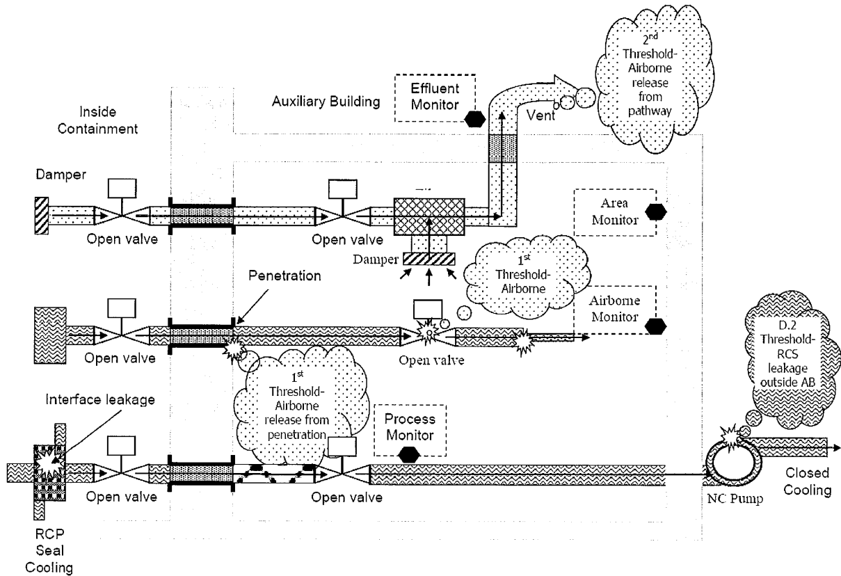
Figure 1: Containment Integrity or Bypass Examples
