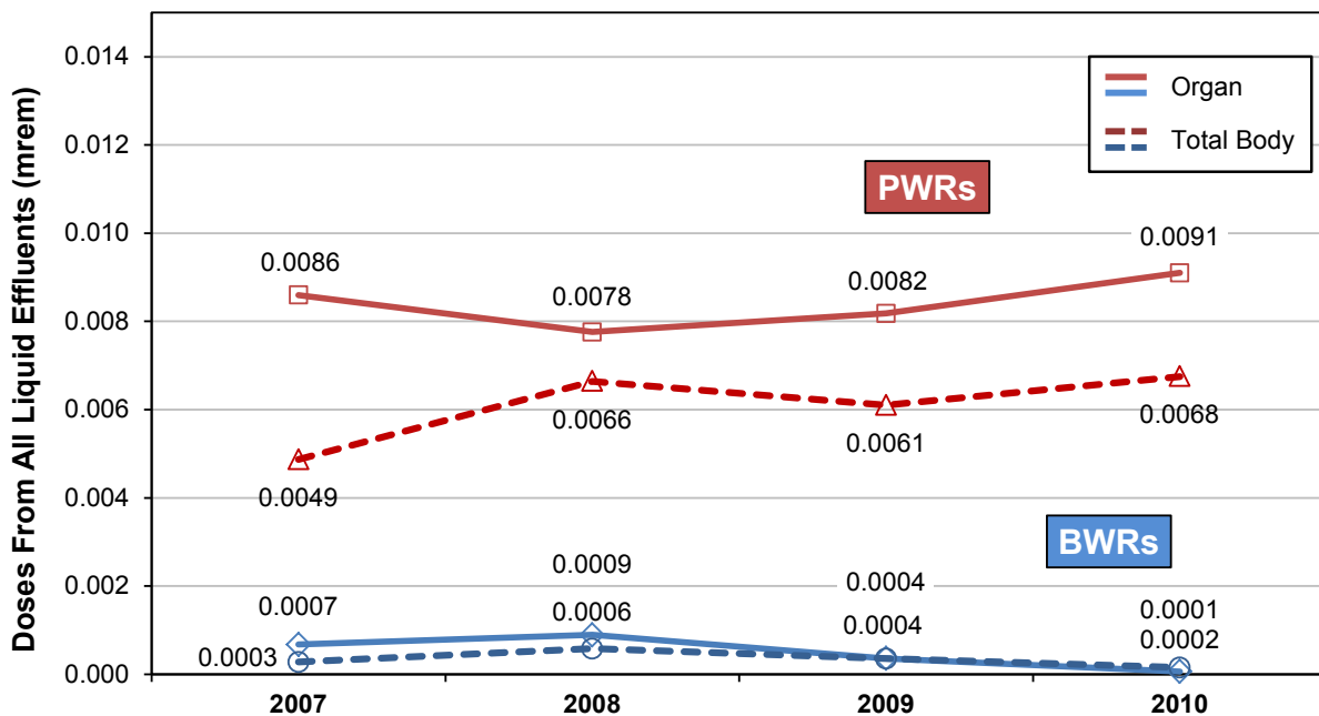
Figure 3.22 Median Maximum Annual Dose, Liquid Effluents 4-Year Trend, 2007-2010
