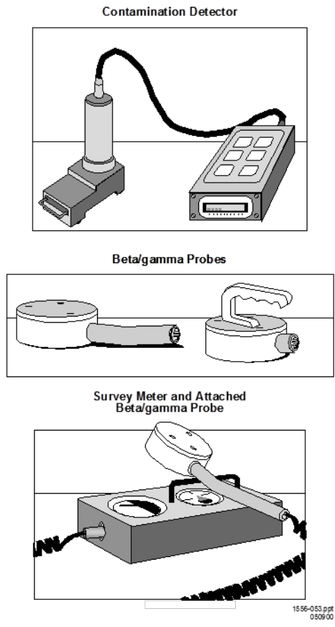
Figure 8-5. Examples of Portable Instruments Used in Laboratory Settings
