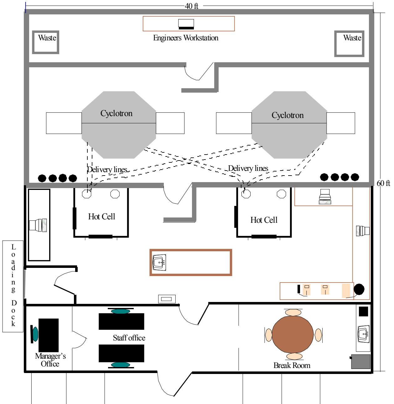
Figure 8-4. Facility Diagram for a Radioactive Materials Production Facility
