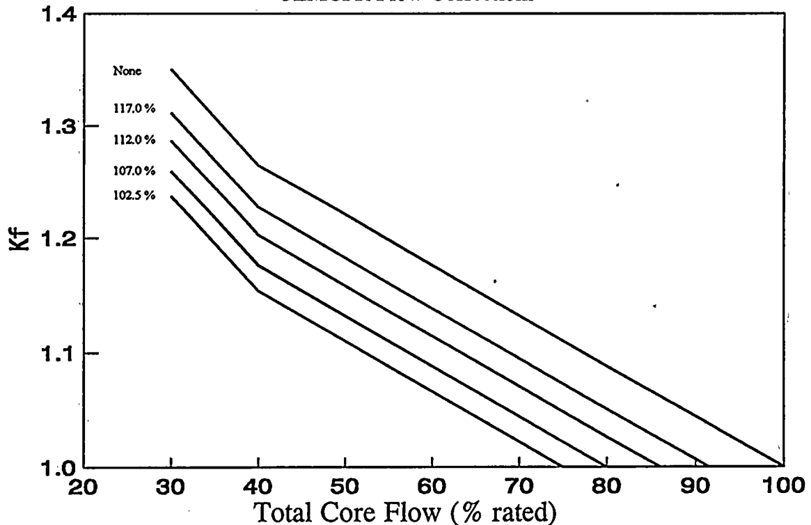
Figure 4 GEXL-Plus K_f Curve OLMCPR Flow Corrections
