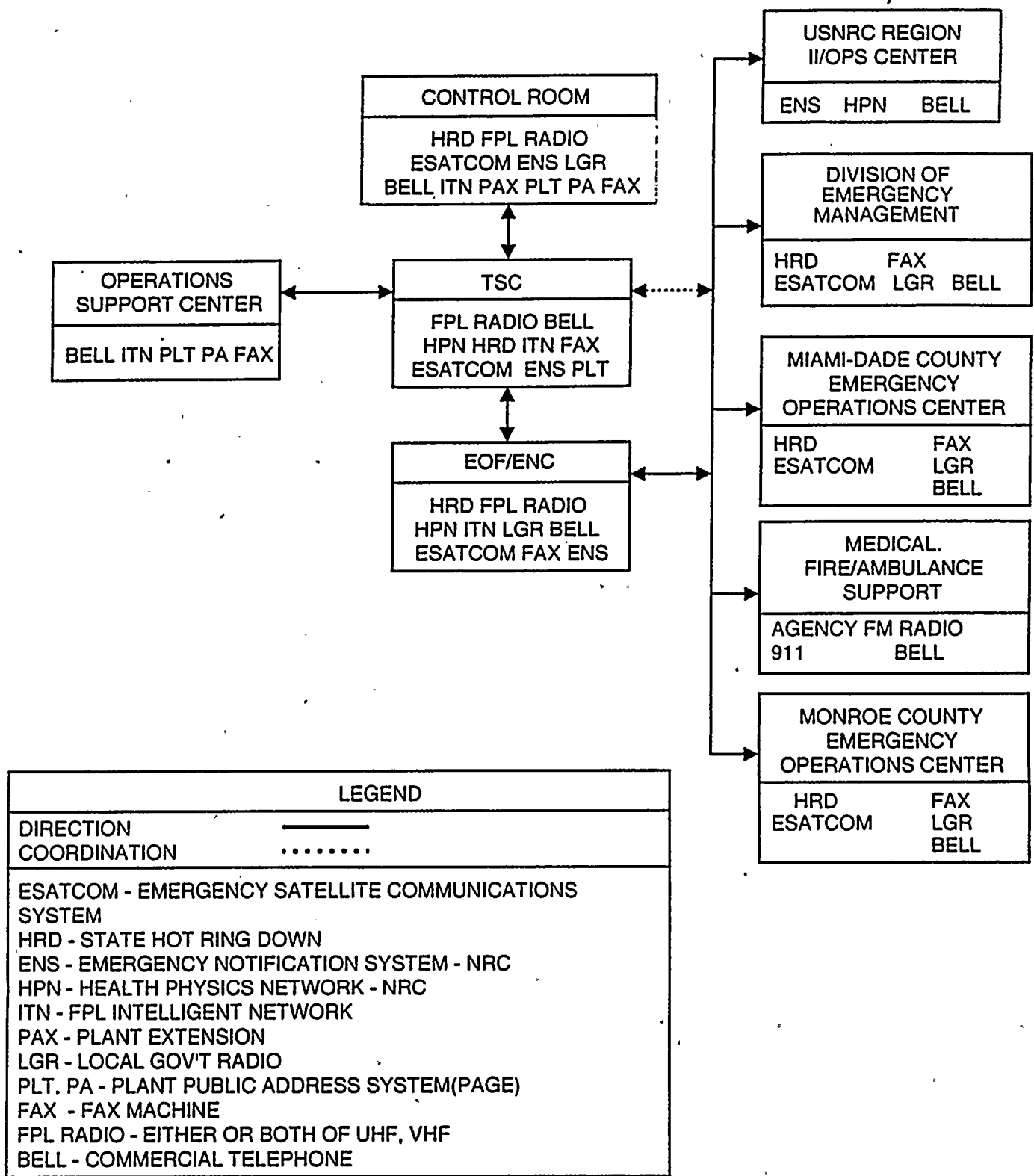
FIGURE 4-1 COMMUNICATIONS INTERFACES
