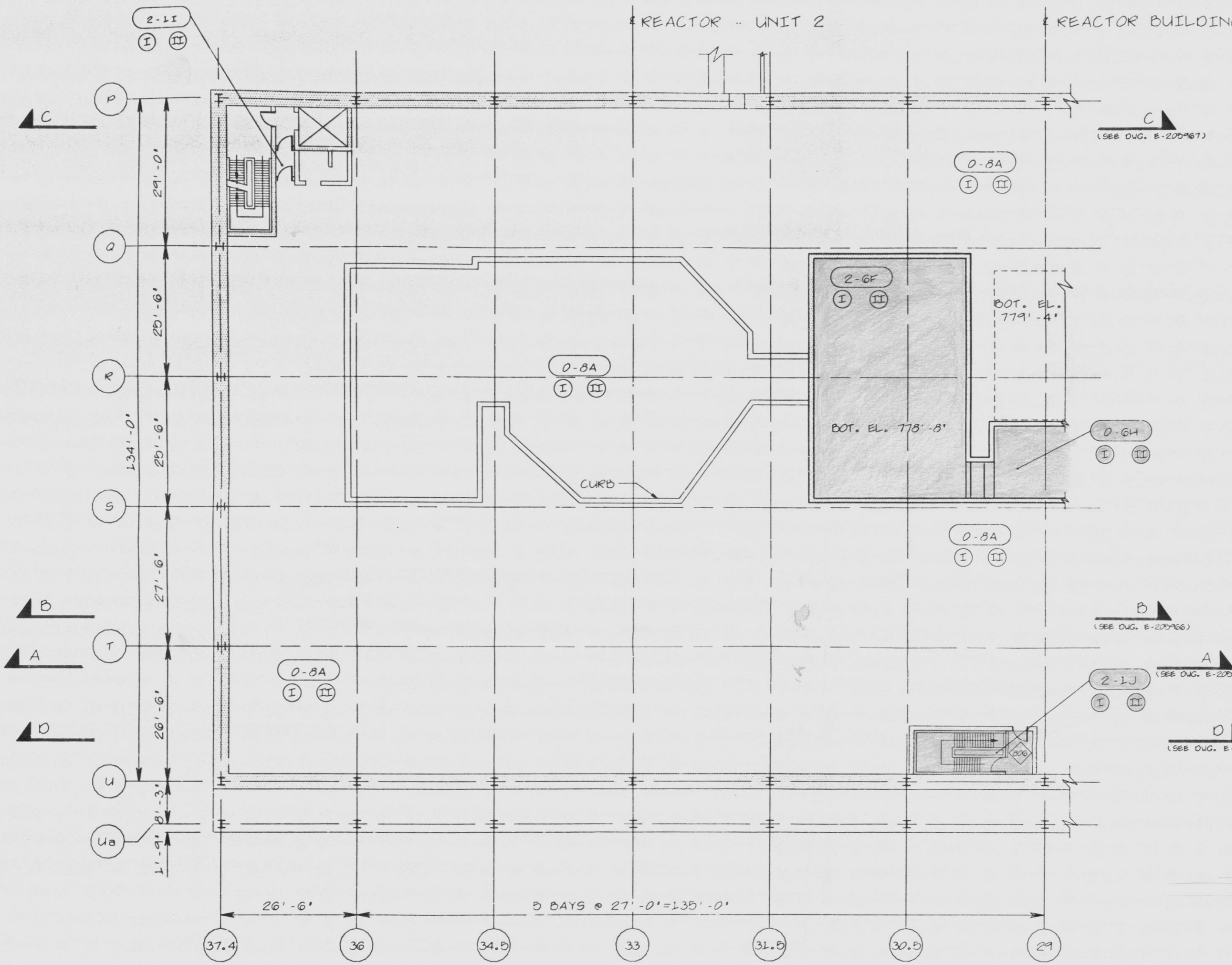
FLOOR PLAN @ EL. 818'-1"
