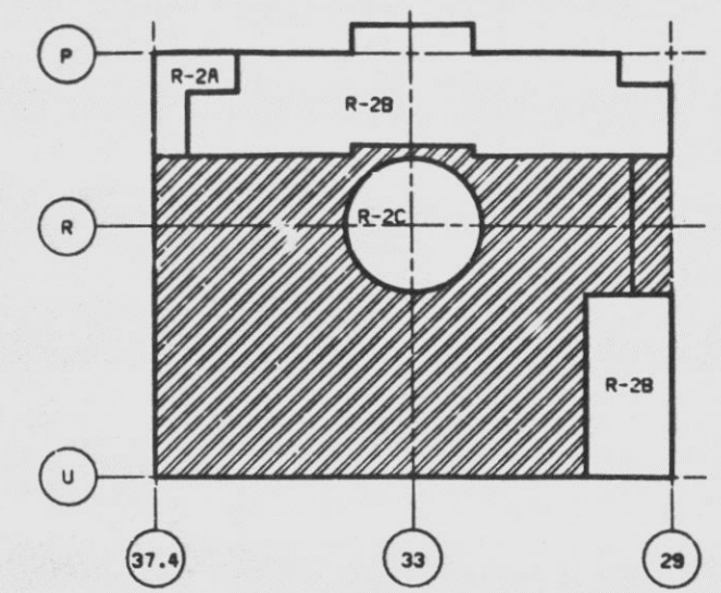
FIRE AREA KEY PLAN ■ BUFFER ZONE
