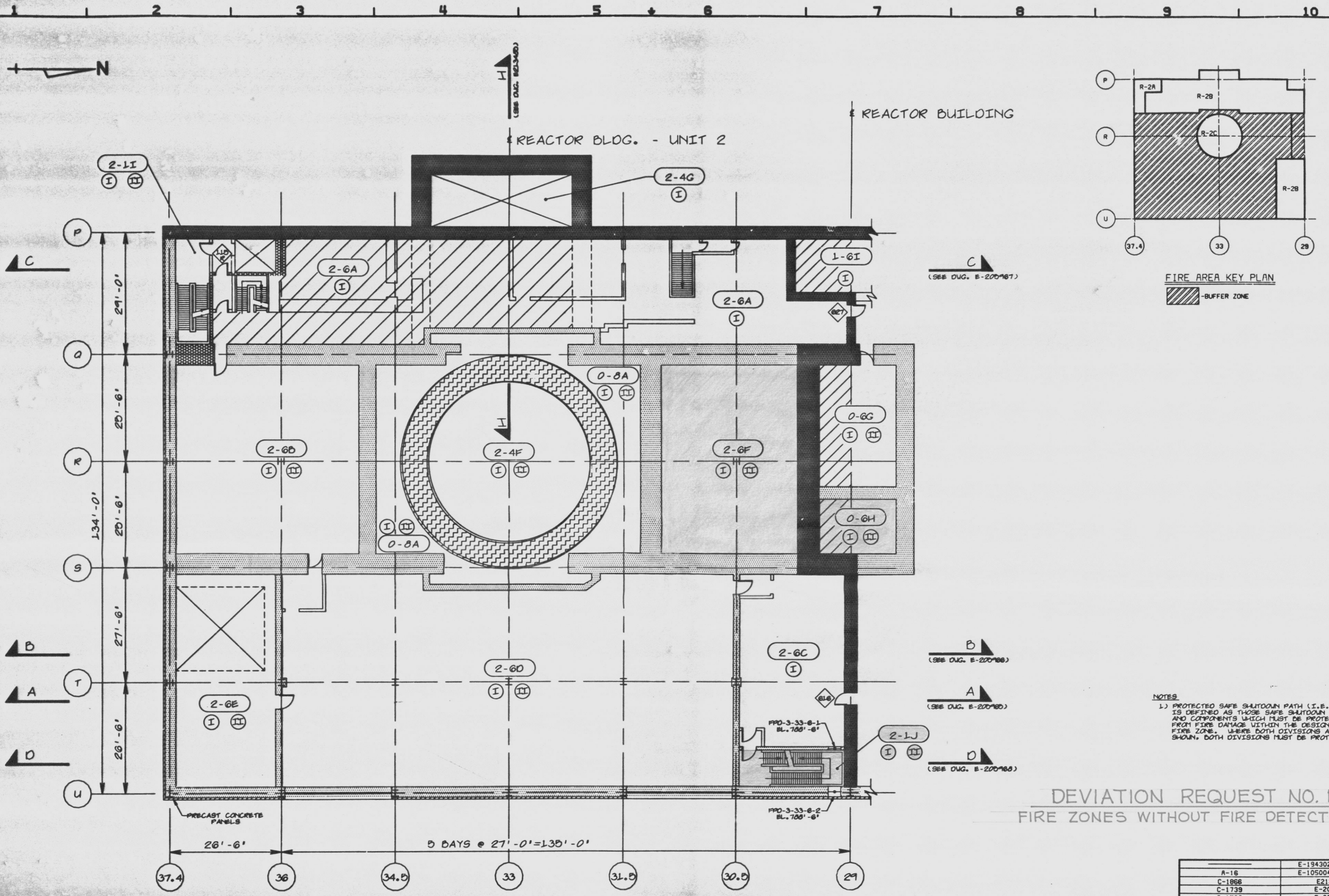
FLOOR PLAN @ EL. 779'-1"
