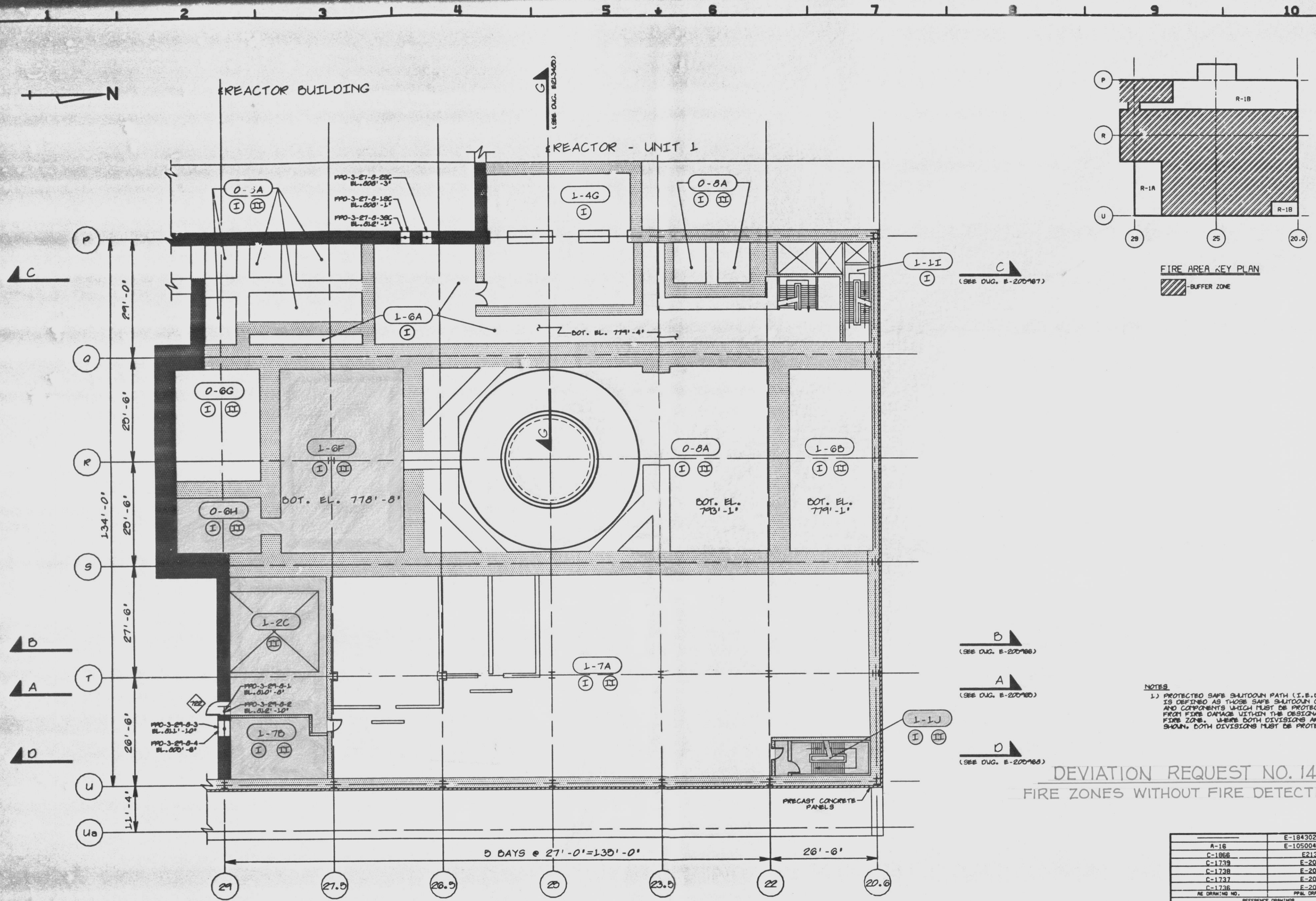
FLOOR PLAN @ EL. 799'-1"
