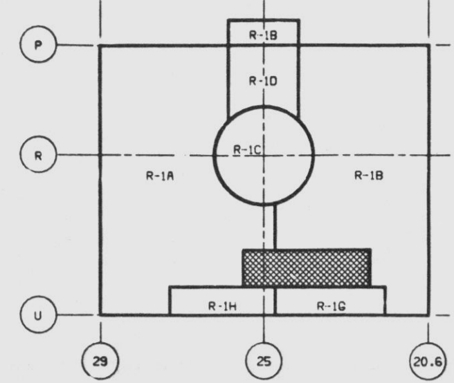
FIRE AREA KEY PLAN HATCHED AREA
