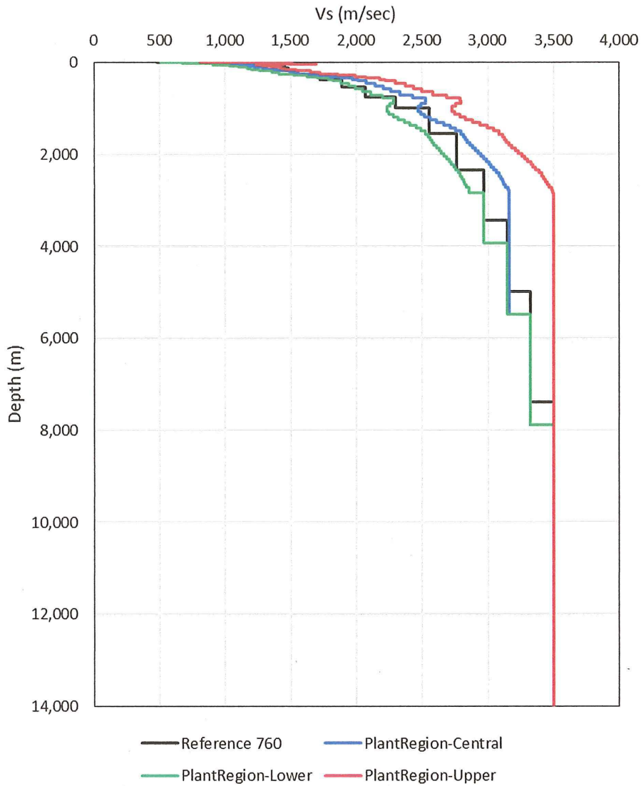
Figure 2-3 - Comparison of the Host VS Profile (labeled Reference 760) and the Central, Upper, and Lower Profiles for the Target (From Reference 8)
