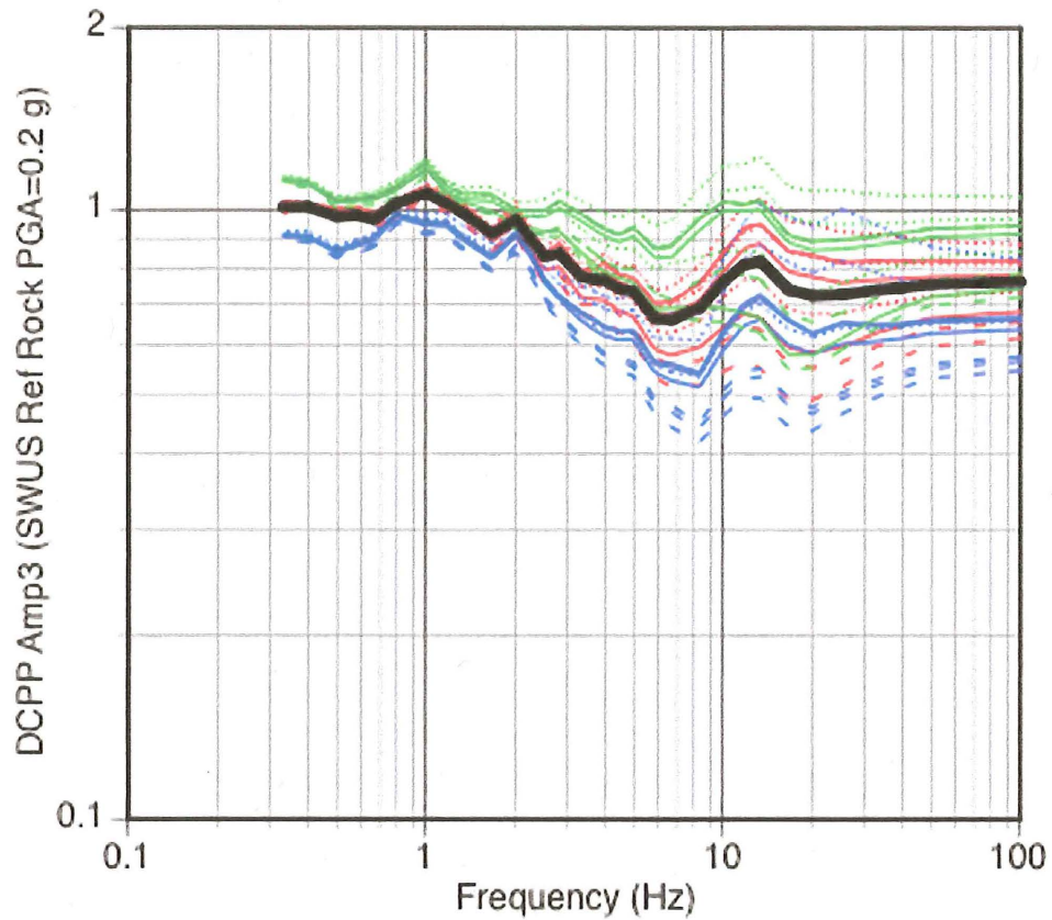
Figure 3-7 - Analytical Site Terms for a SWUS Reference Rock (760 m/s) PGA of 0.2 g
