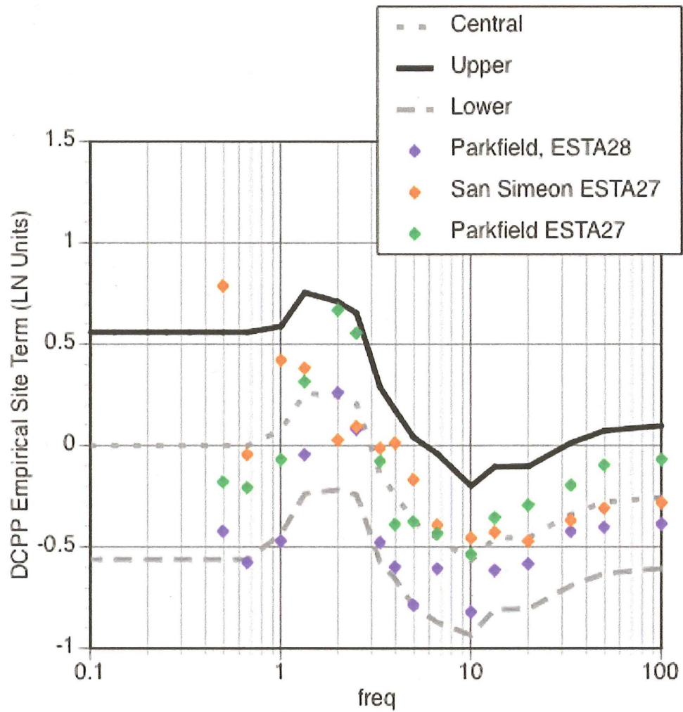
Figure 4-2 - Empirical Site Term for DCPD Relative to SWUS Reference Rock (From Reference 9)
