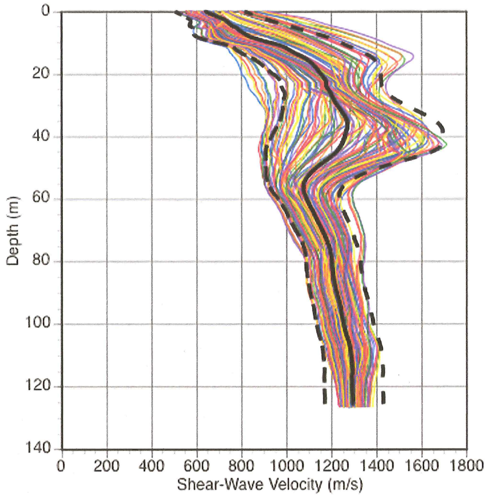
Figure 2-2 - Range of VS Profiles Under the Power-Block and Turbine Building Region in the Top 125 m
