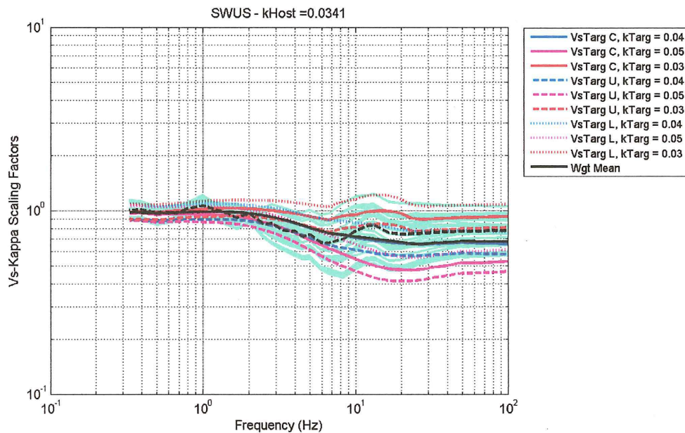
Figure 2-6 - VS-Kappa Factors from the Best Kappa from IRVT (colored curves) and from Analytical Modeling (cyan curves). The mean for the analytical model is given by dashed black line. The mean for the IRVT method is shown by the solid black line. (From Reference 10)
