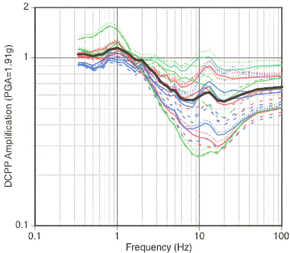
Figure 3-9 - Analytical site terms for a SWUS reference rock (760 m/s) PGA of 1.91 g, corresponding to the 1E-5 hazard level.
