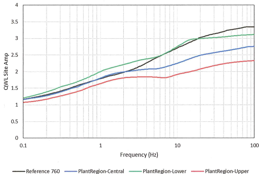
Figure 2-5 - Quarter Wave-Length Crustal Amplification Factors (Fourier Amplitude Spectra Amplification) for the Host VS profile and the Central, Upper, and Lower Target VS Profiles (From GEO.DCPP.15.03 (Reference 10))
