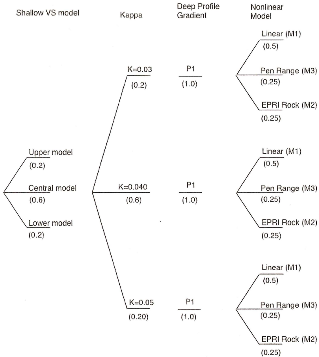
Figure 3-2 - Logic Tree for Inputs to Analytical Site Response
