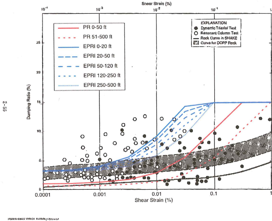
Figure 3-6 - 1978 Lab Testing for Nonlinear Damping for DCP Rock
