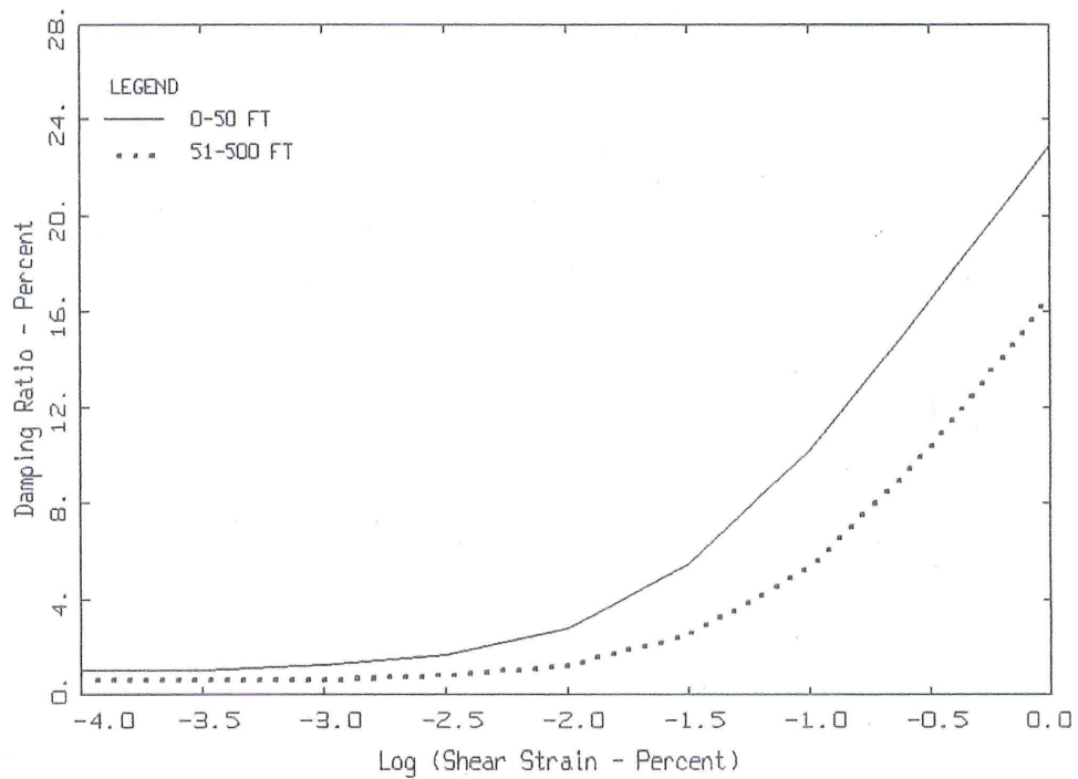
PENINSULAR RANGE MODULUS REDUCTION AND DAMPING CURVES
