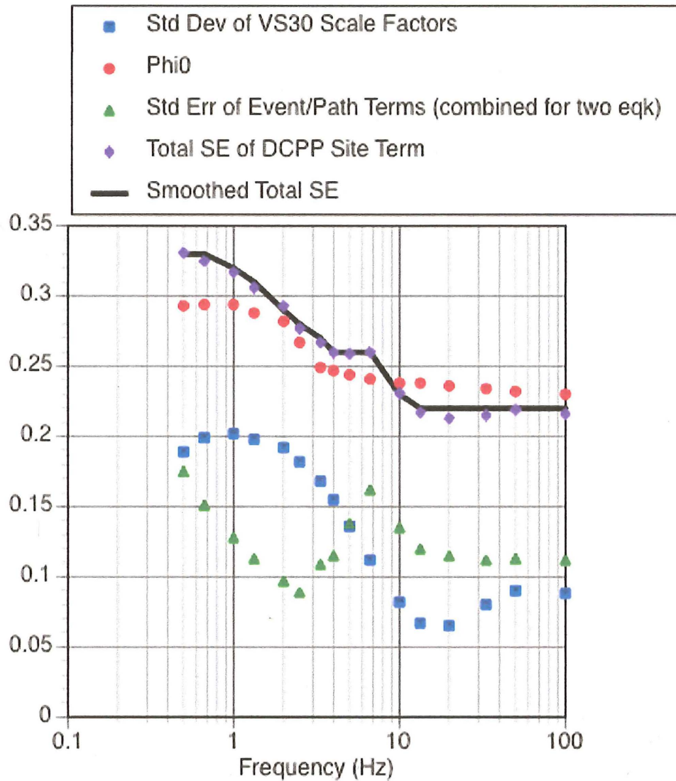
Figure 4-1 - Empirical Site Term for DCPD Relative to SWUS Reference Rock (From Reference 9)
