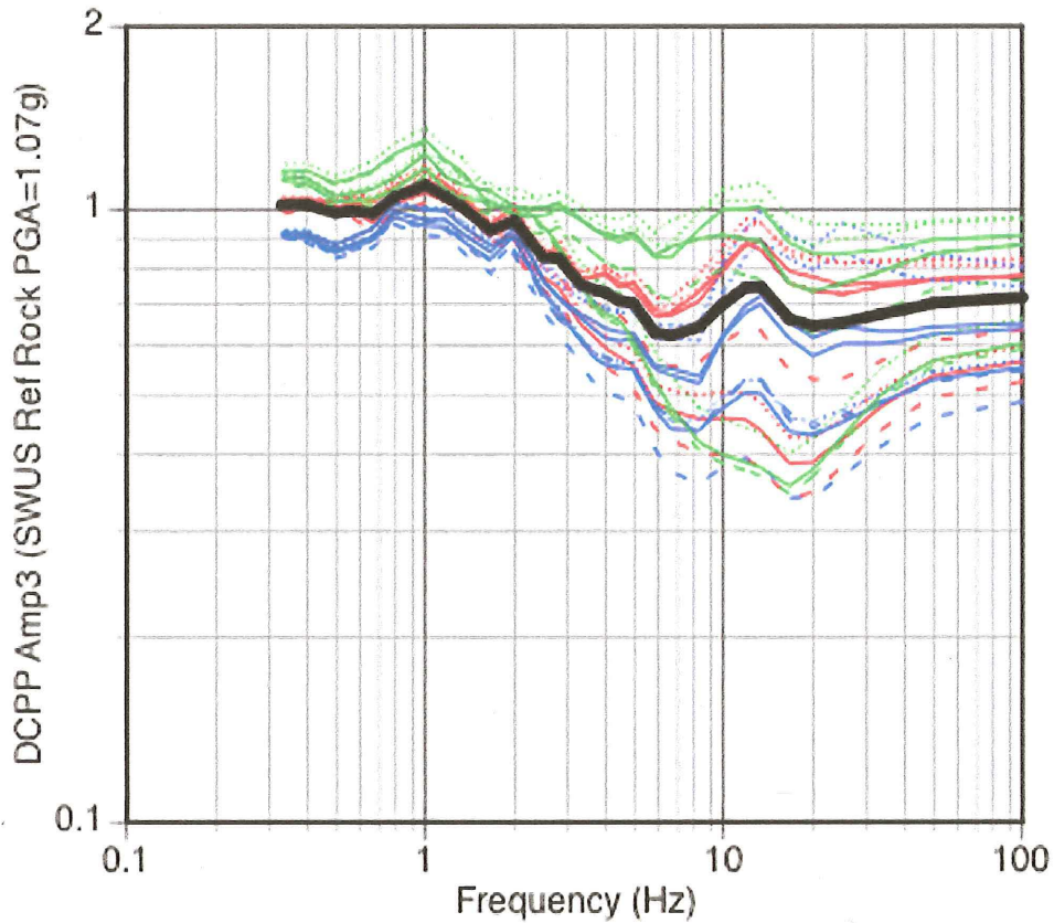
Figure 3-8 - Analytical site terms for a SWUS reference rock (760 m/s) PGA of 1.07 g
