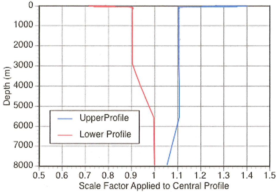
Figure 2-4b - Scale Factors used to Develop the Upper and Lower VS Profiles for the Full Depth Range (From Table A-3)
