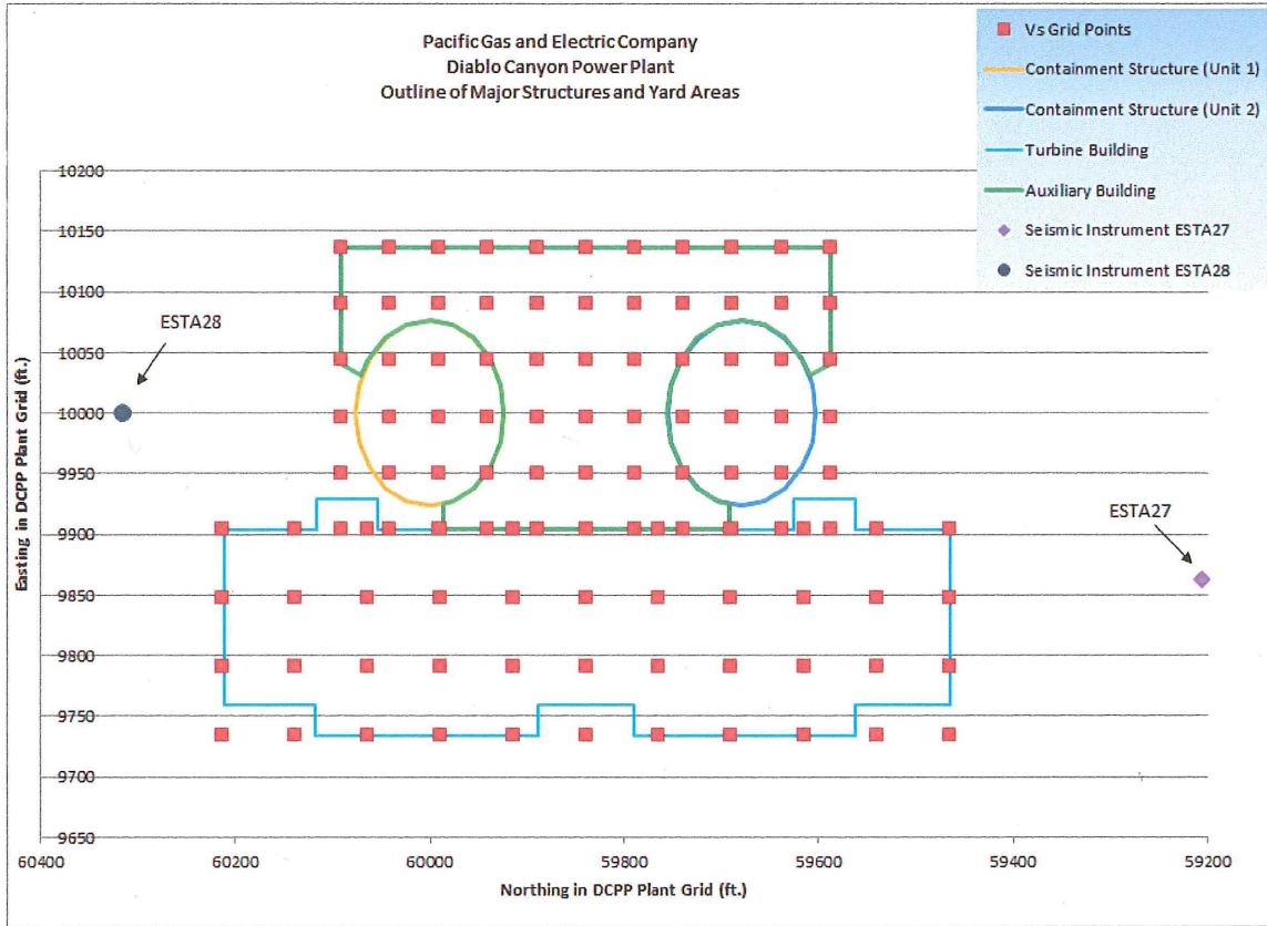
Figure 2-1 - Locations of 1-D Profiles used to Define the Power-Block and Turbine Building Region
