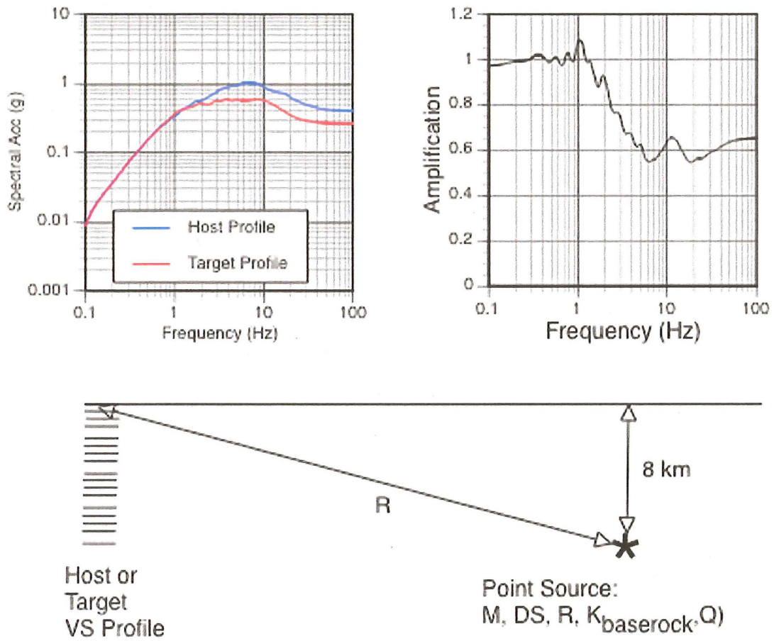
Figure 3-1 - Cartoon of the Analytical Site Response
