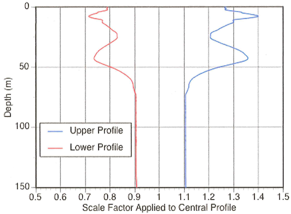
Figure 2-4a - Scale Factors used to Develop the Upper and Lower VS Profiles for the top 150 m (From Table A-3)
