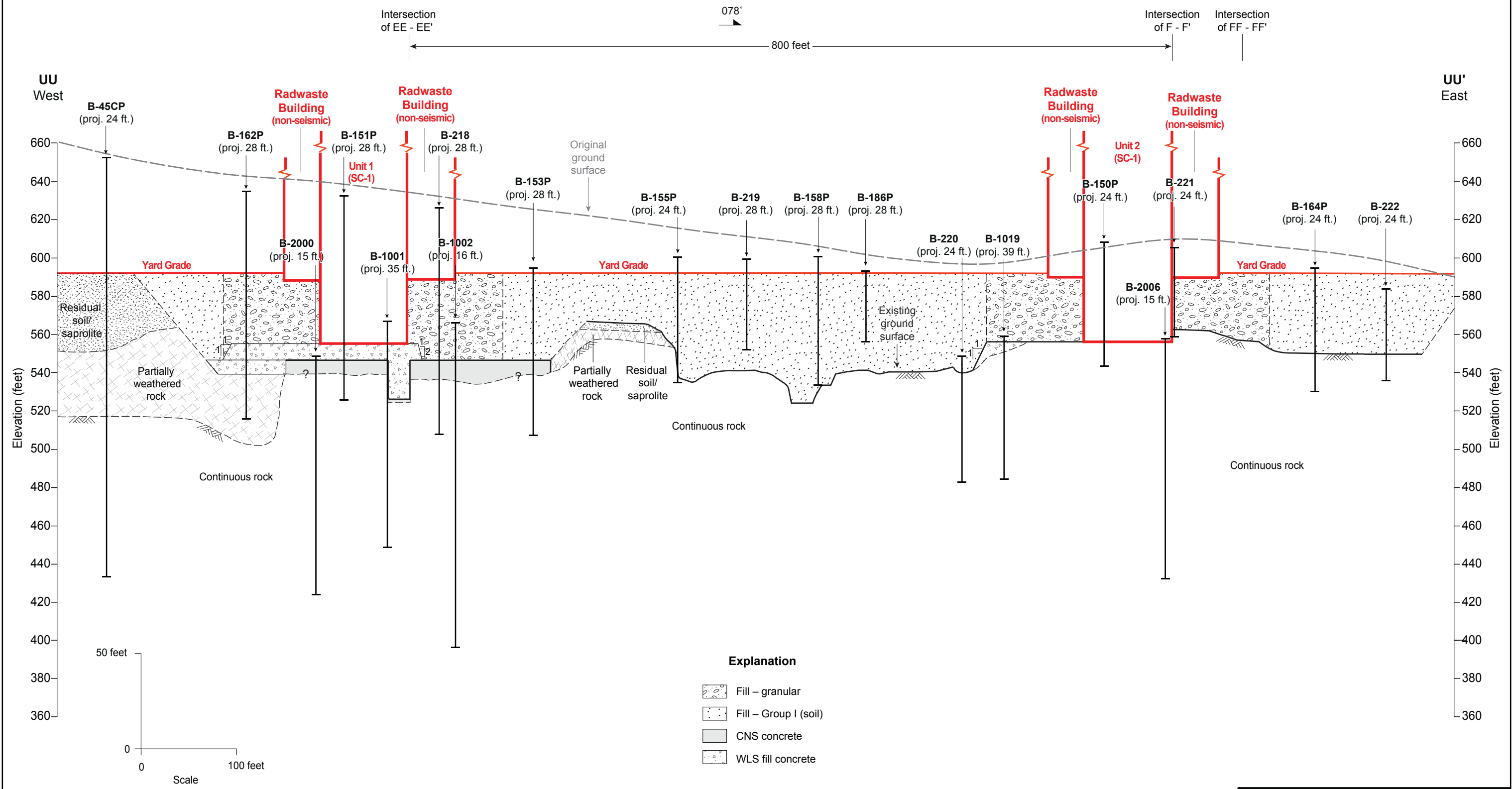
WILLIAM STATES LEE III NUCLEAR STATION UNITS 1 & 2 Planned Excavation Profile, Geologic Cross Section UU-UU' FIGURE 2.5.4-245 Rev 9
