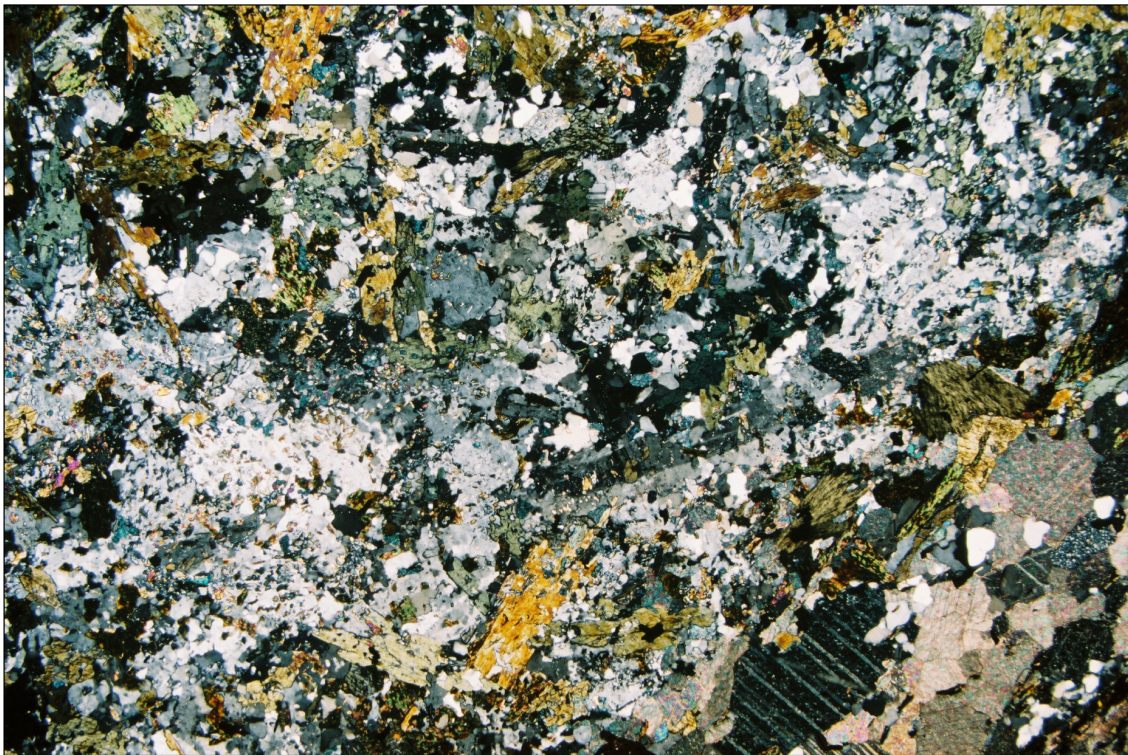
Meta-basalt showing typical appearance of fine equigranular texture and a vein (lower right) of ferroan calcite + chlorite + quartz + K-Spar
