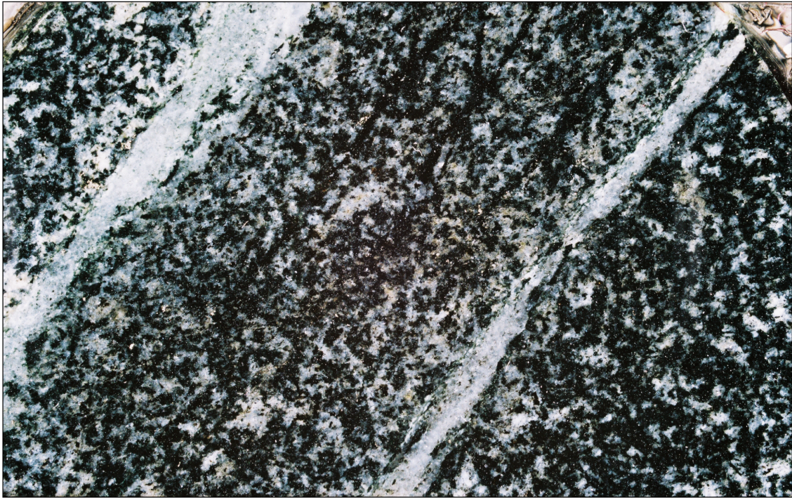
Meta-basalt showing typical appearance of hand specimen with two kinds of veins
