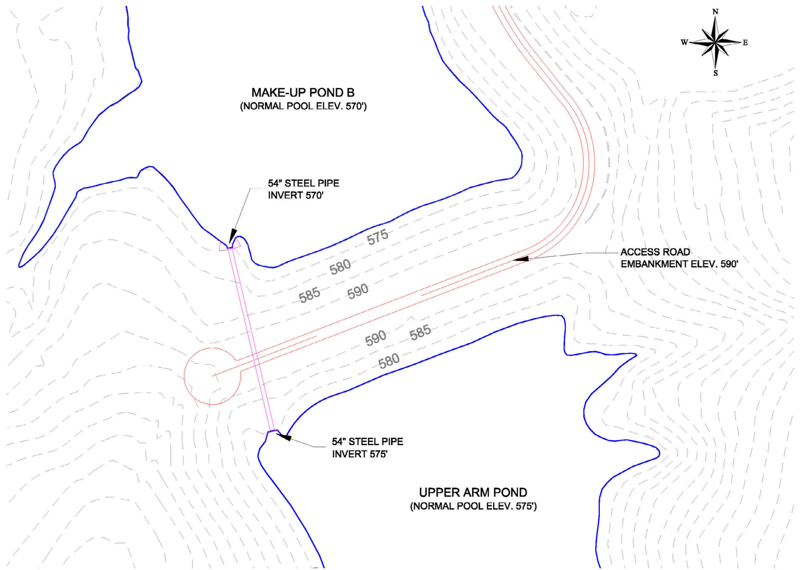
WILLIAM STATES LEE III NUCLEAR STATION UNITS 1 & 2 Drainage Culvert Schematic, Upper Arm Dam FIGURE 2.4.3-249 Rev 6
