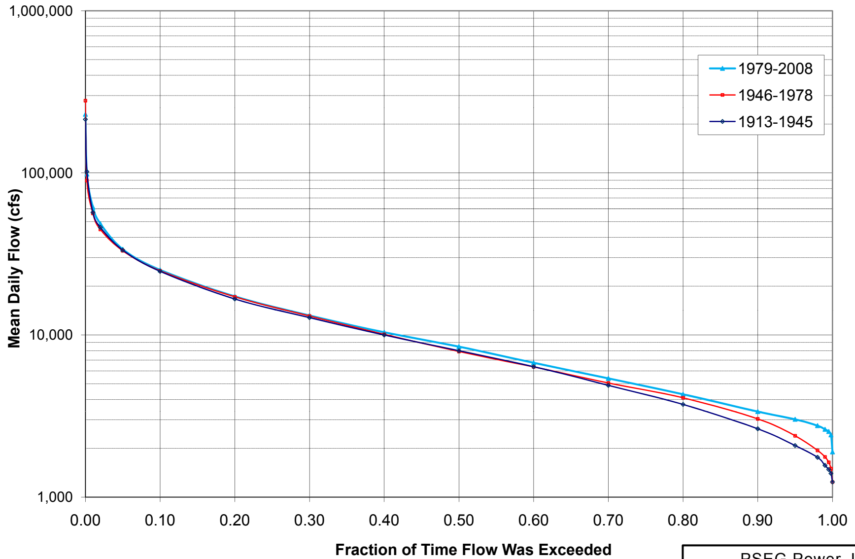
PSEG Power, LLC PSEG Site ESPA Part 3, Environmental Report Daily Mean Flow Duration Curves – Delaware River at Trenton NJ FIGURE 2.3-3
