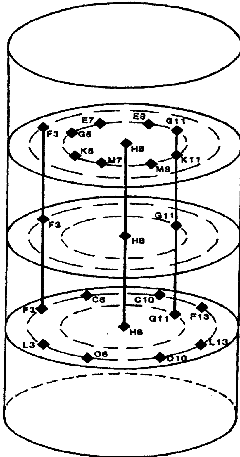
INCORE INSTRUMENTATION SPECIFICATION THREE MILE ISLAND NUCLEAR STATION UNIT 1
