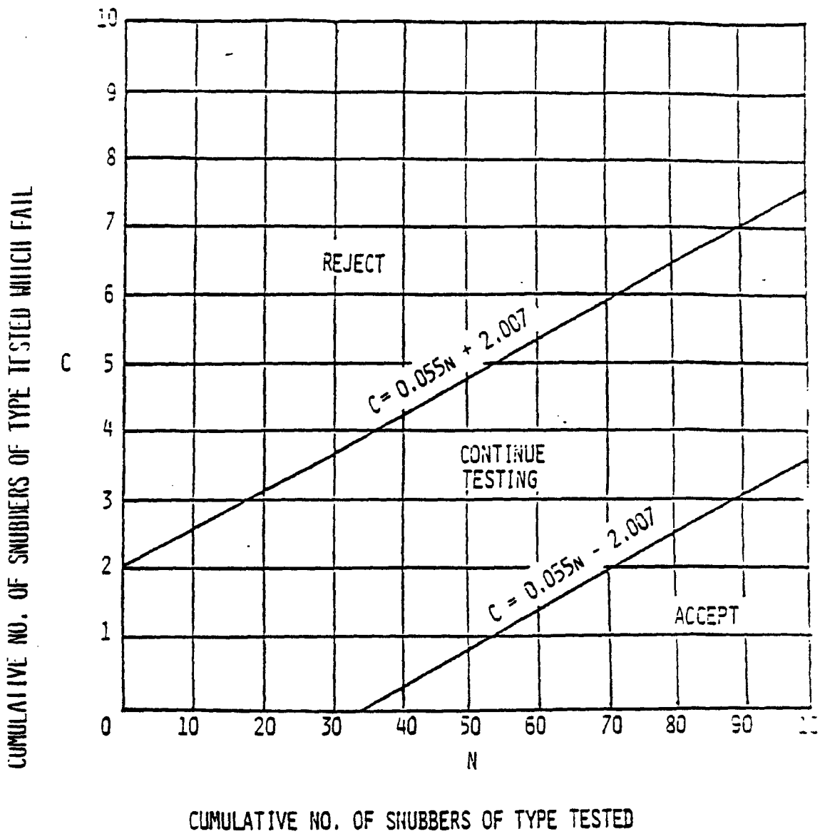
FIGURE 4.17-1 SNUBBER FUNCTIONAL TEST - SAMPLE PLAN 2
