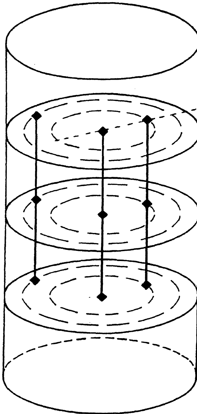
INCORE INSTRUMENTATION SPECIFICATION AXIAL IMBALANCE INDICATION THREE MILE ISLAND NUCLEAR STATION UNIT 1
