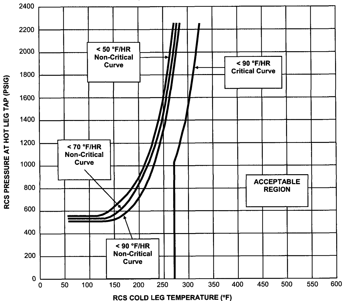
FIGURE 3.4.3-1 RCS Heatup Limitations to 5434 EFPY
