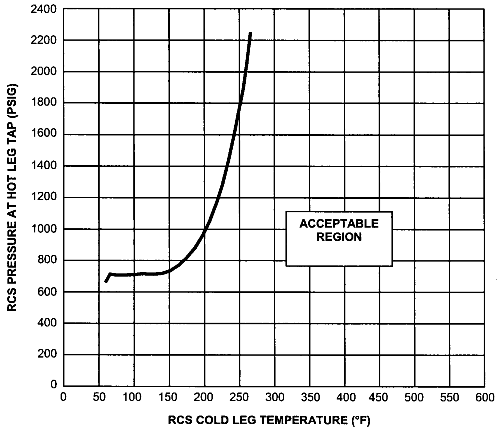
FIGURE 3.4.3-3 RCS Inservice Hydrostatic Test H/U & C/D Limits to 5434 EFPY
