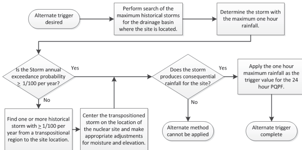
Figure 2. Alternate Action Trigger Flowchart
