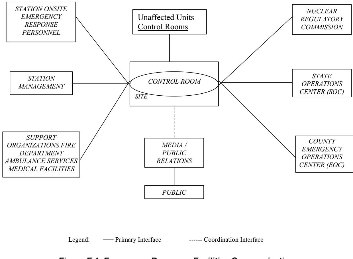
Figure F-1 Emergency Response Facilities Communications Pathway Typical Functional Diagram Unusual Event
