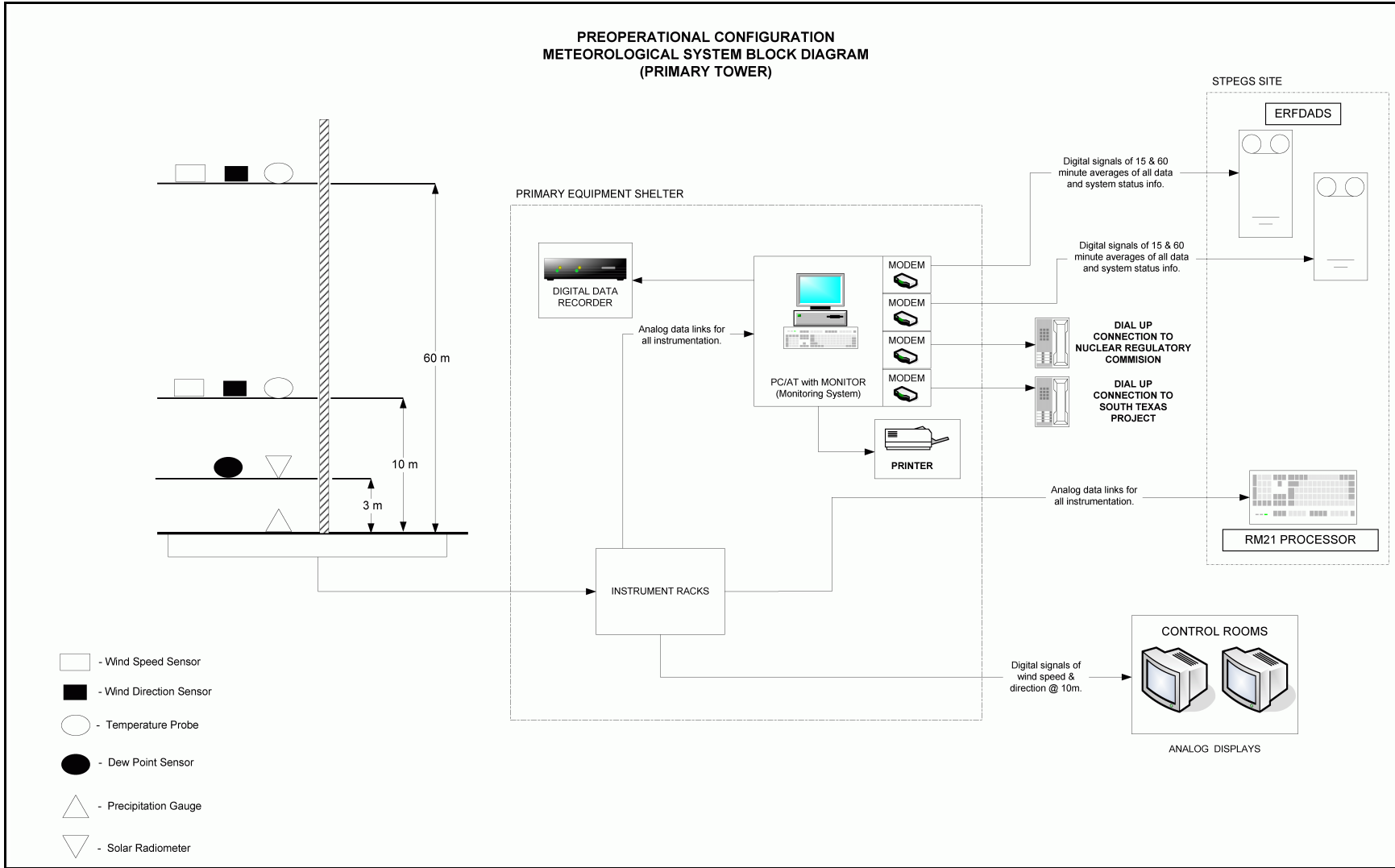
Figure 6.4-5 Meteorological System Block Diagram (Primary Tower – Preoperational Configuration)
