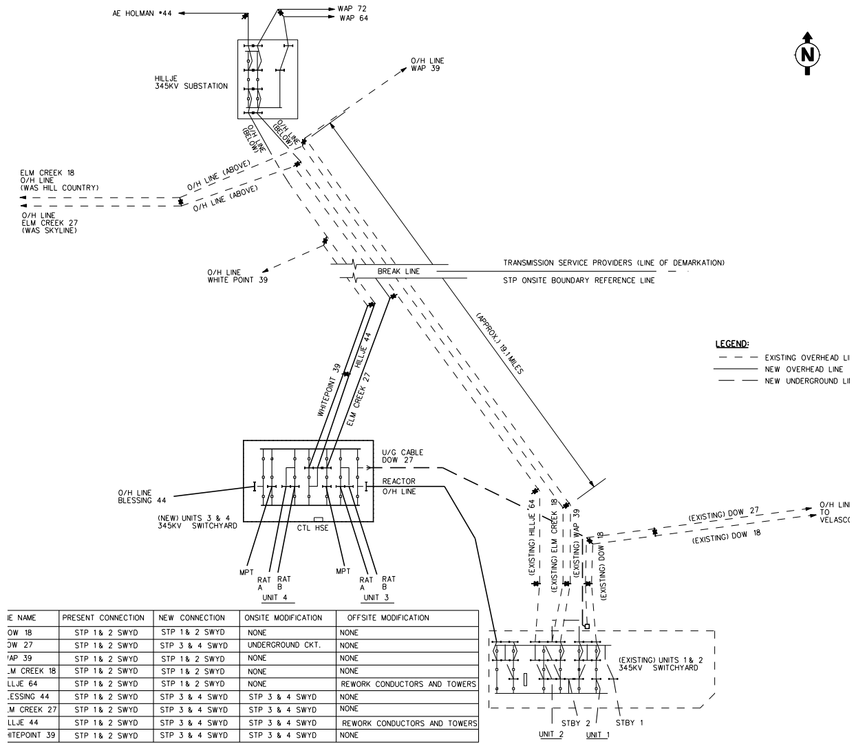
Figure 3.7-5 345kV Transmission Configuration for STP 1 & 2 and STP 3 & 4
