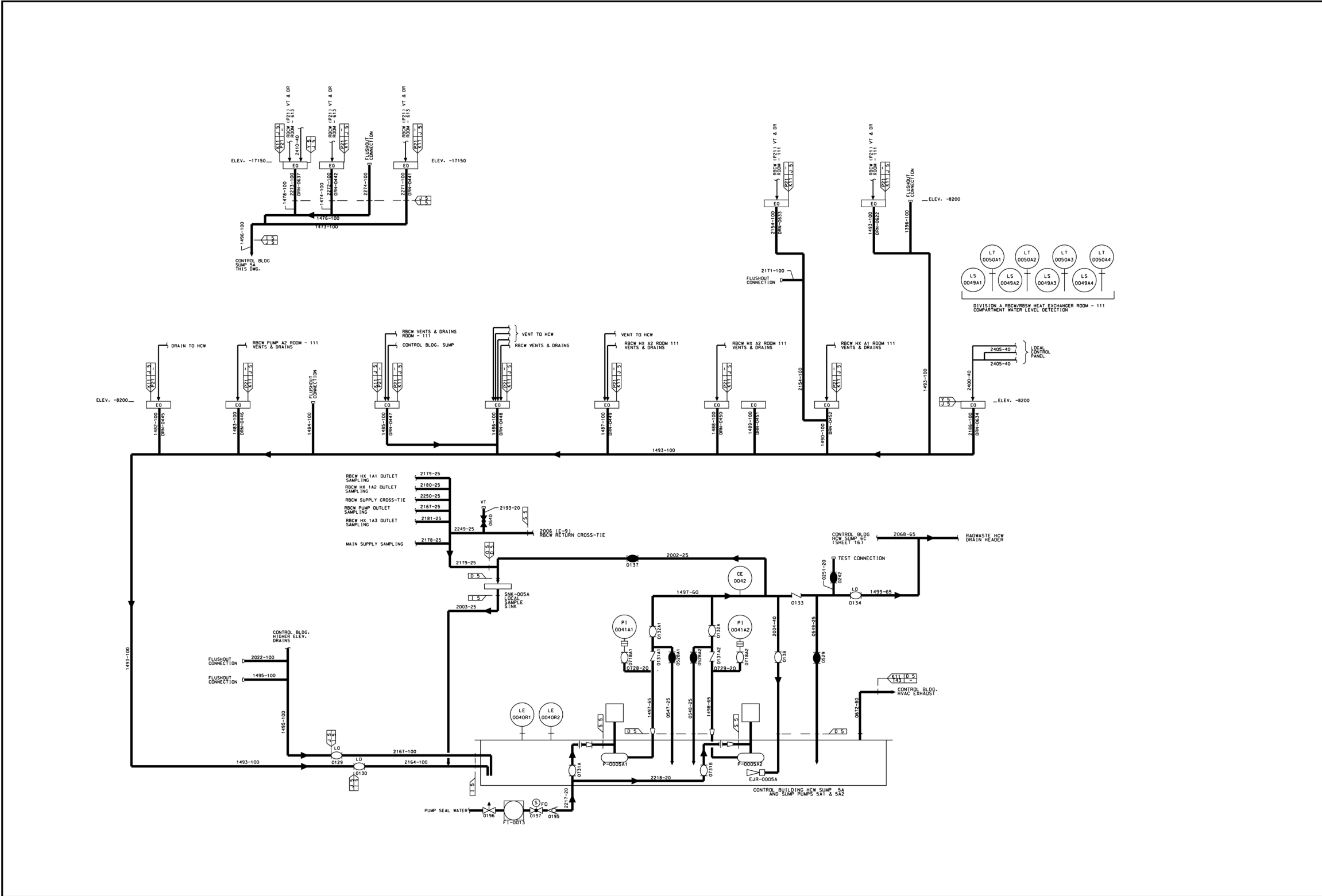
Figure 9.3-11 – Piping and Instrumentation Diagram, Radioactive Drain Transfer (Sheet 14 of 22)
