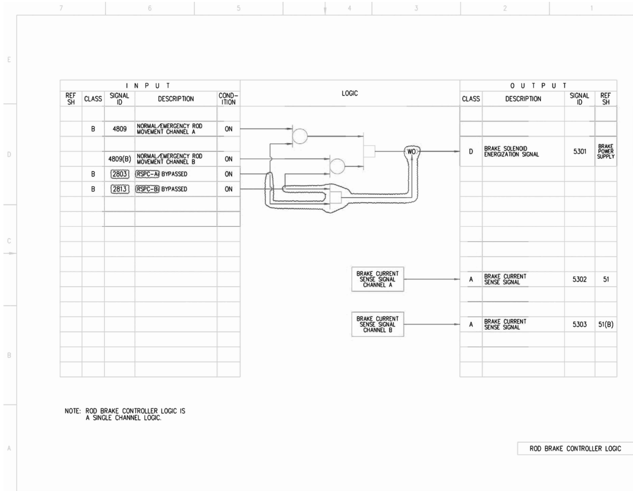
Figure 7.7-3 – Rod Control and Information System IBD (Sheet 53 of 87)
