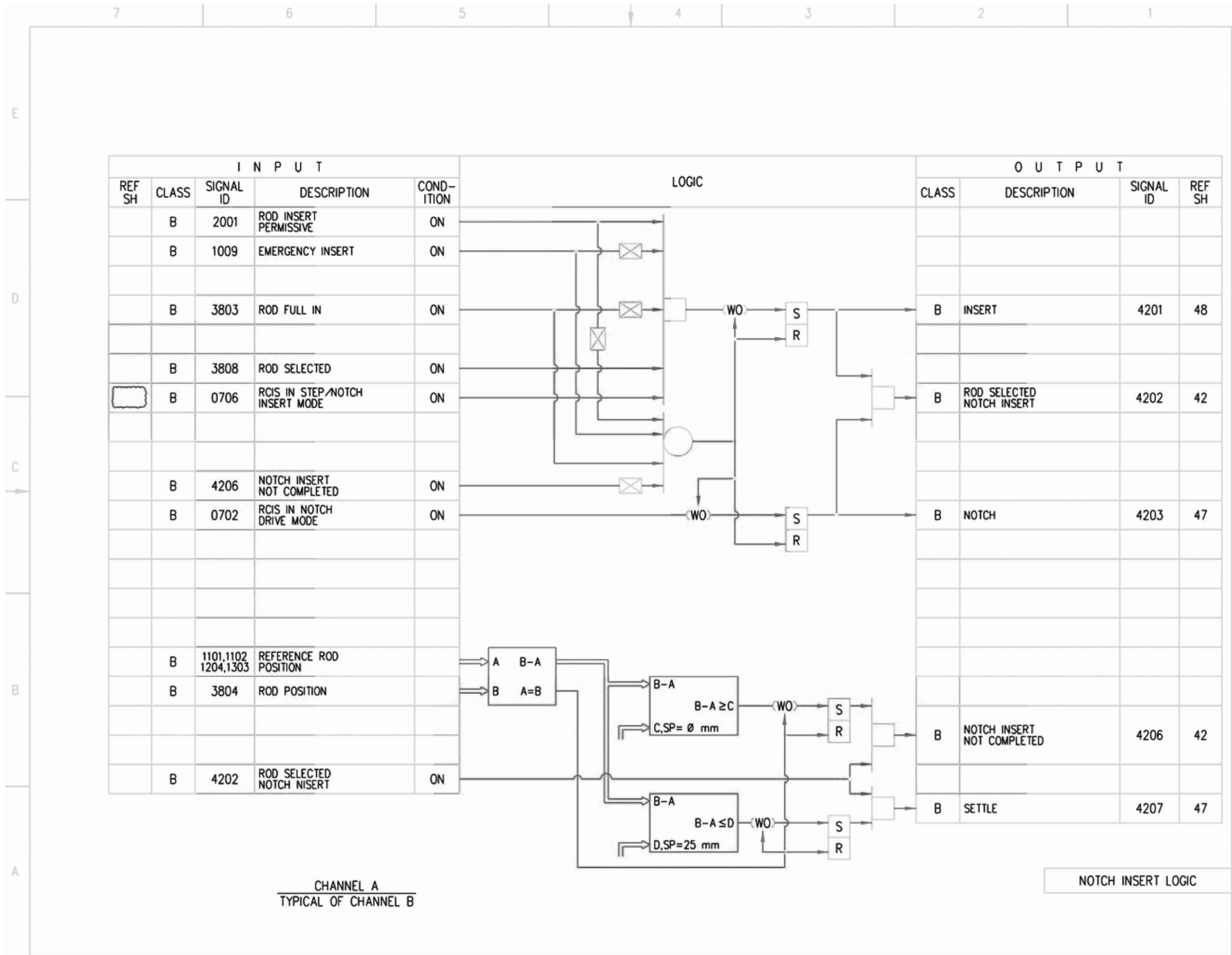
Figure 7.7-3 – Rod Control and Information System IBD (Sheet 42 of 87)
