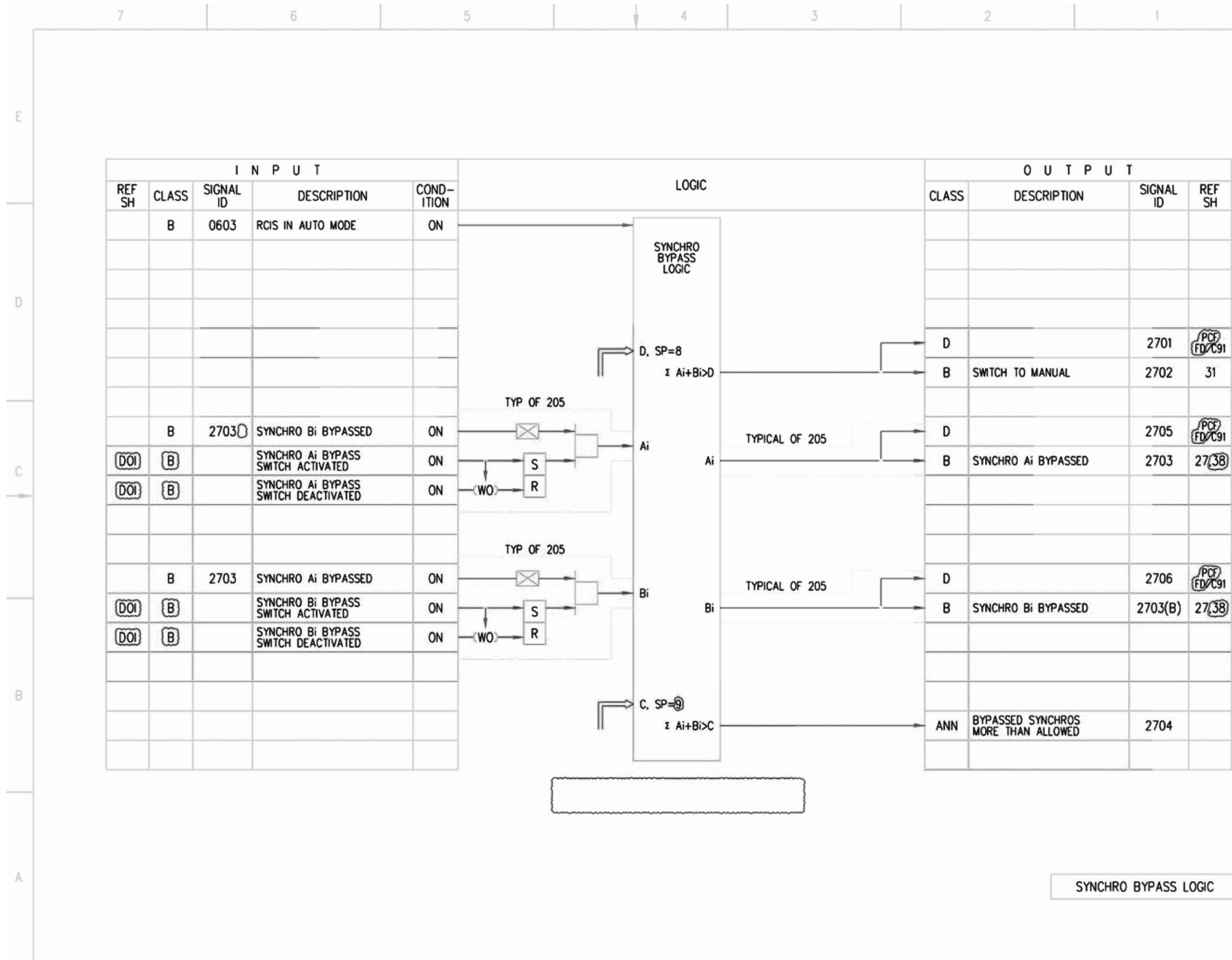
Figure 7.7-3 – Rod Control and Information System IBD (Sheet 27 of 87)
