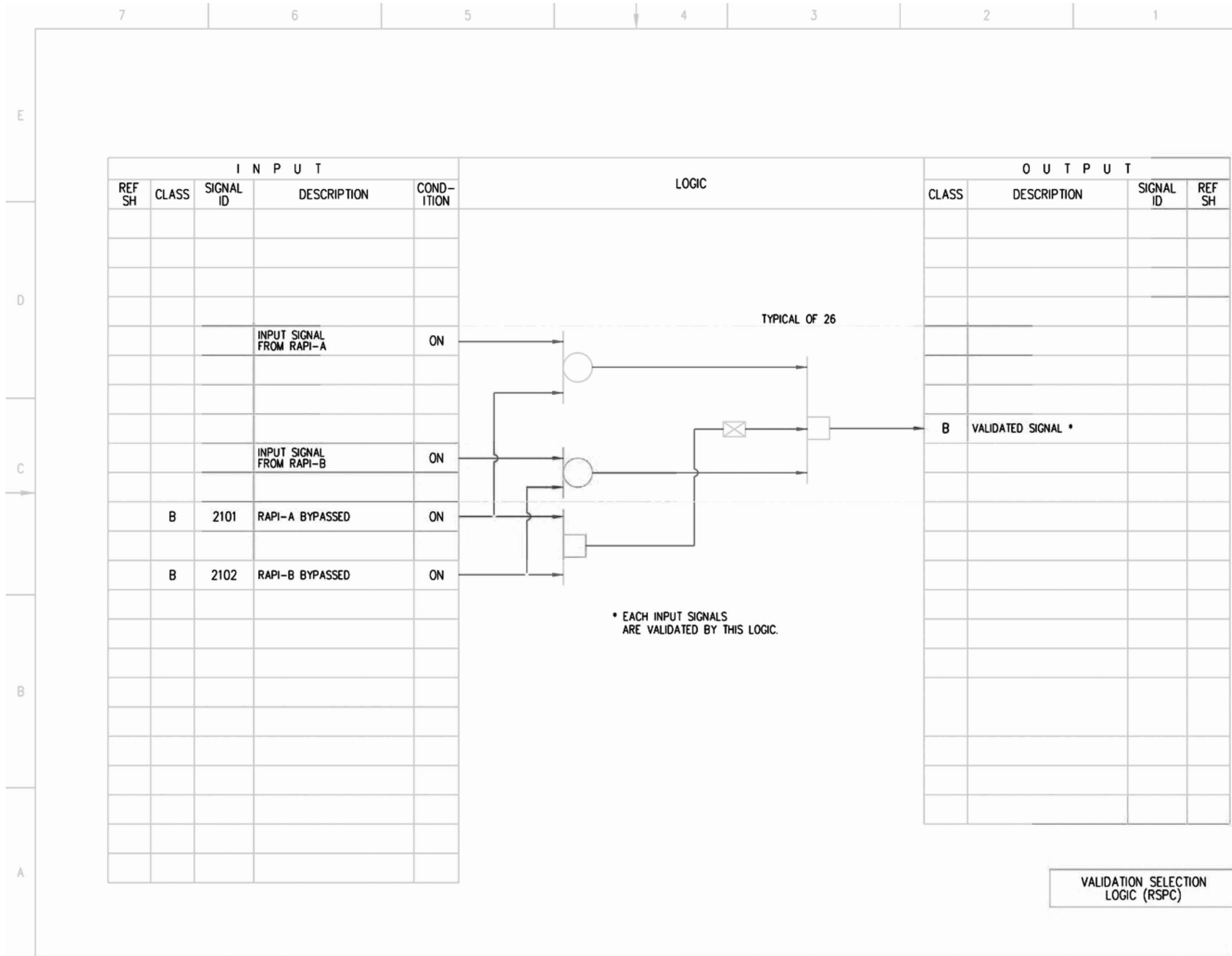
Figure 7.7-3 – Rod Control and Information System IBD (Sheet 37a of 87)
