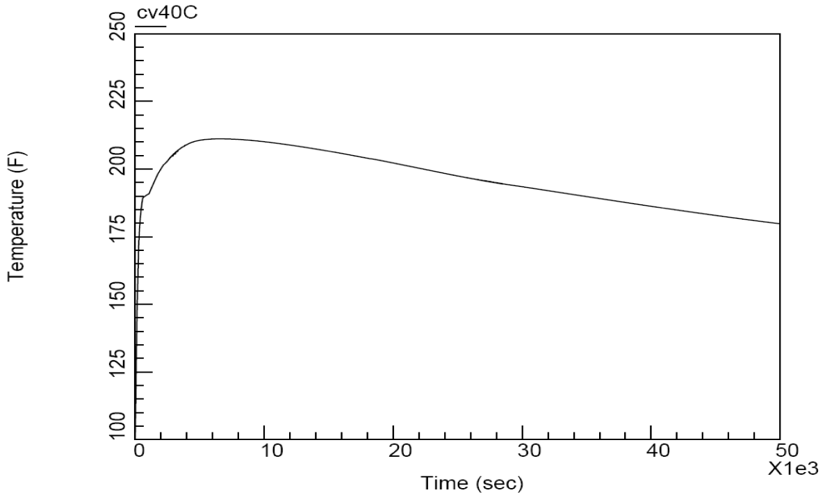
Figure 6.2-13b Suppression Pool Temperature Time History for MSLB
