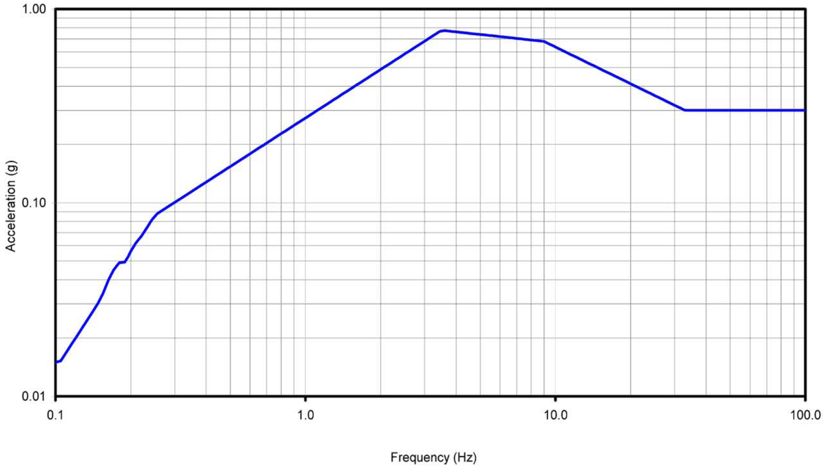
Figure 3.7-39 Vertical Control Building Annex Input Motion for II/I Design (7% Damping)
