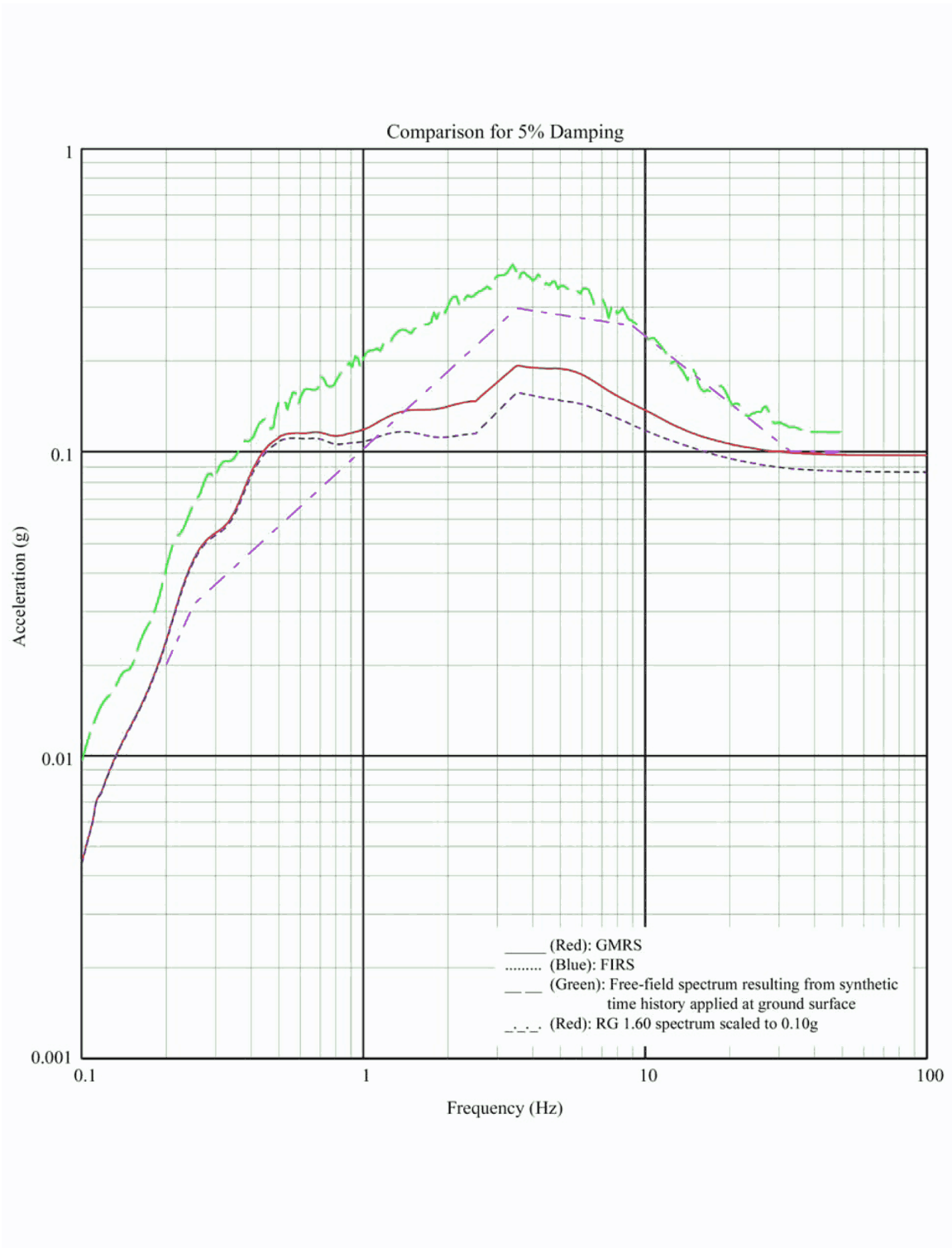
Figure 3A-241 Comparison of Spectra at Foundation of Reactor Building - Lower Bound Soil Properties, Vertical Direction
