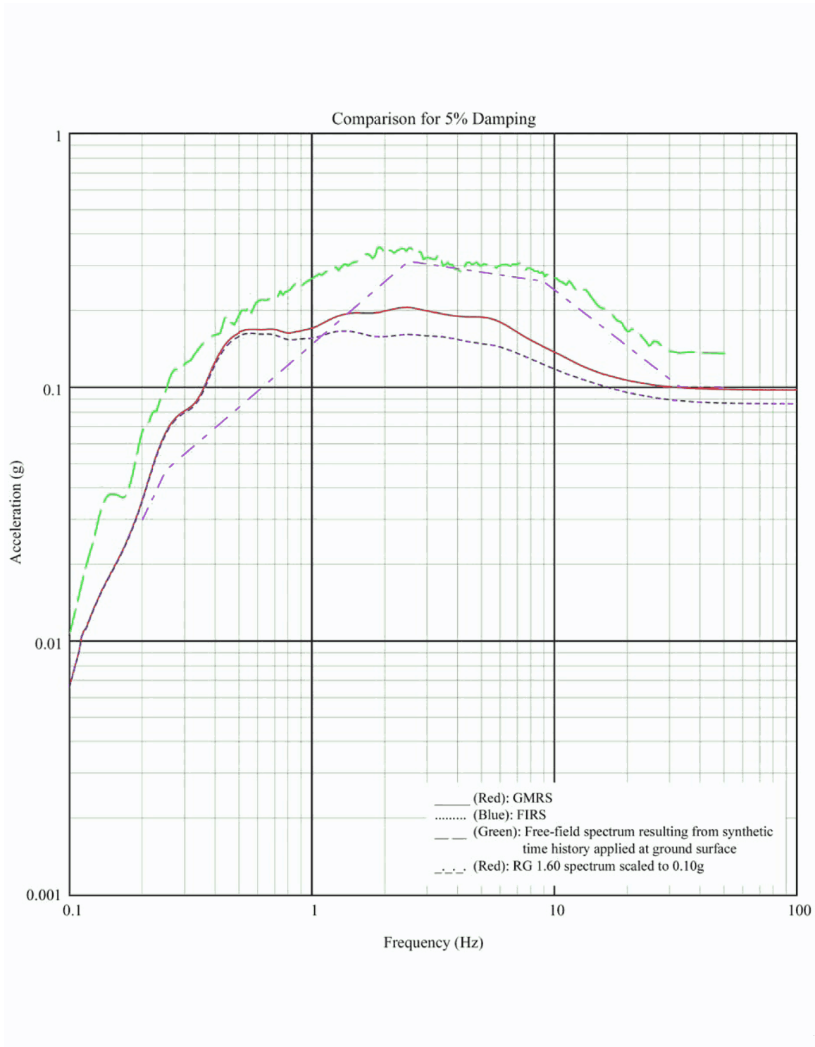
Figure 3A-236 Comparison of Spectra at Foundation of Reactor Building - Upper Bound Soil Properties, X Direction
