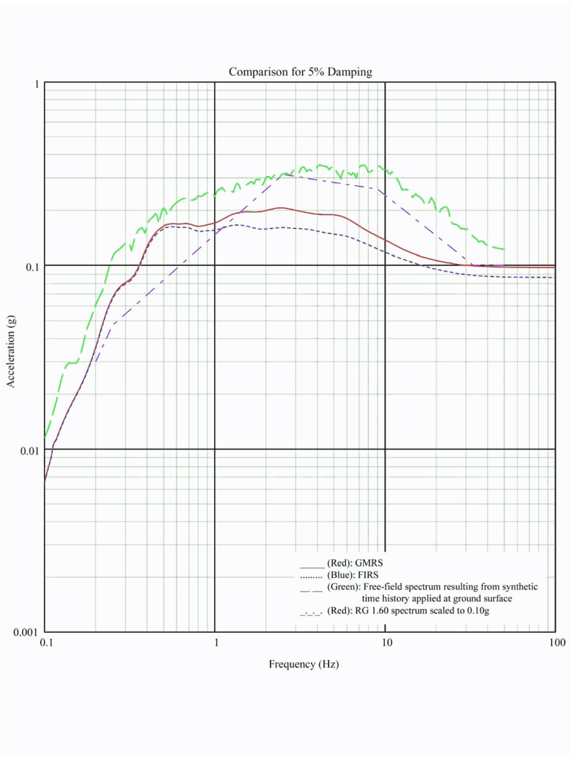
Figure 3A-240 Comparison of Spectra at Foundation of Reactor Building - Lower Bound Soil Properties, Y Direction
