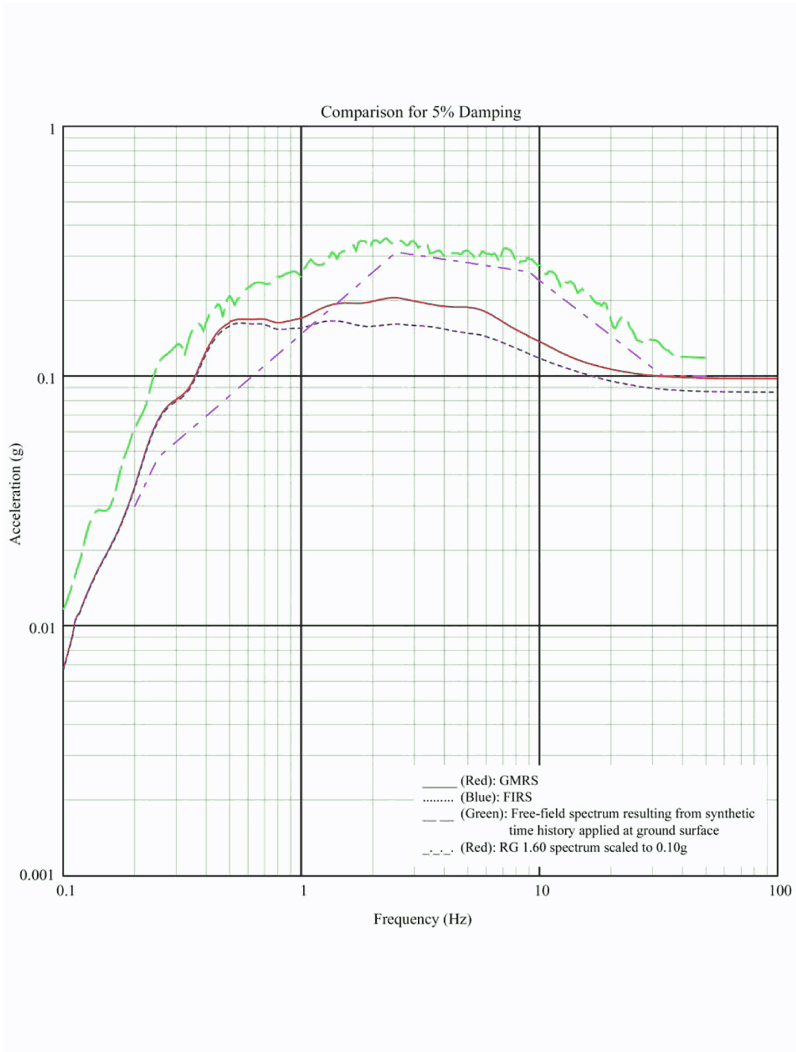
Figure 3A-237 Comparison of Spectra at Foundation of Reactor Building - Upper Bound Soil Properties, Y Direction
