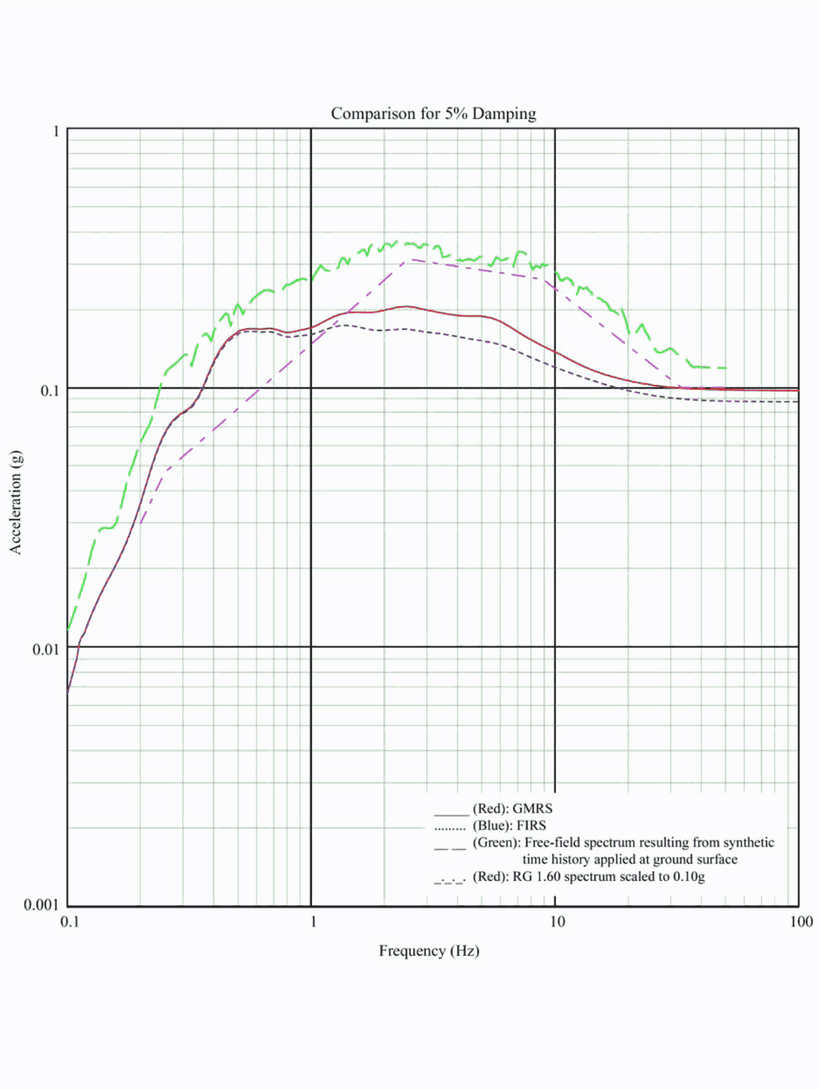
Figure 3A-246 Comparison of Spectra at Foundation of Control Building - Upper Bound Soil Properties, Y Direction
