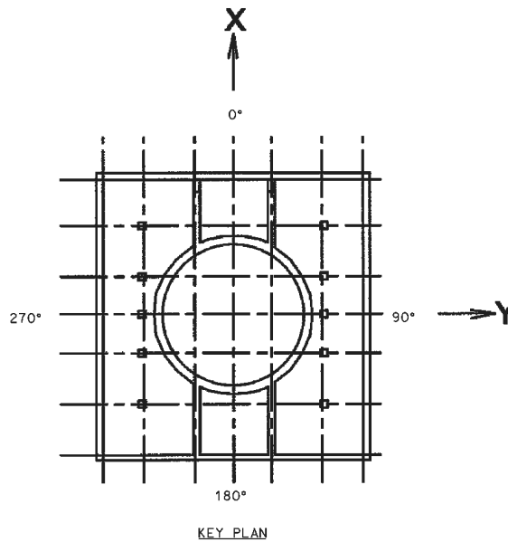
Figure 3A-229 Reactor Building Key Plan and Section
