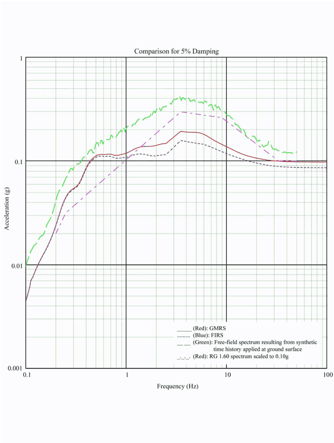
Figure 3A-235 Comparison of Spectra at Foundation of Reactor Building - Mean Soil Properties, Vertical Direction
