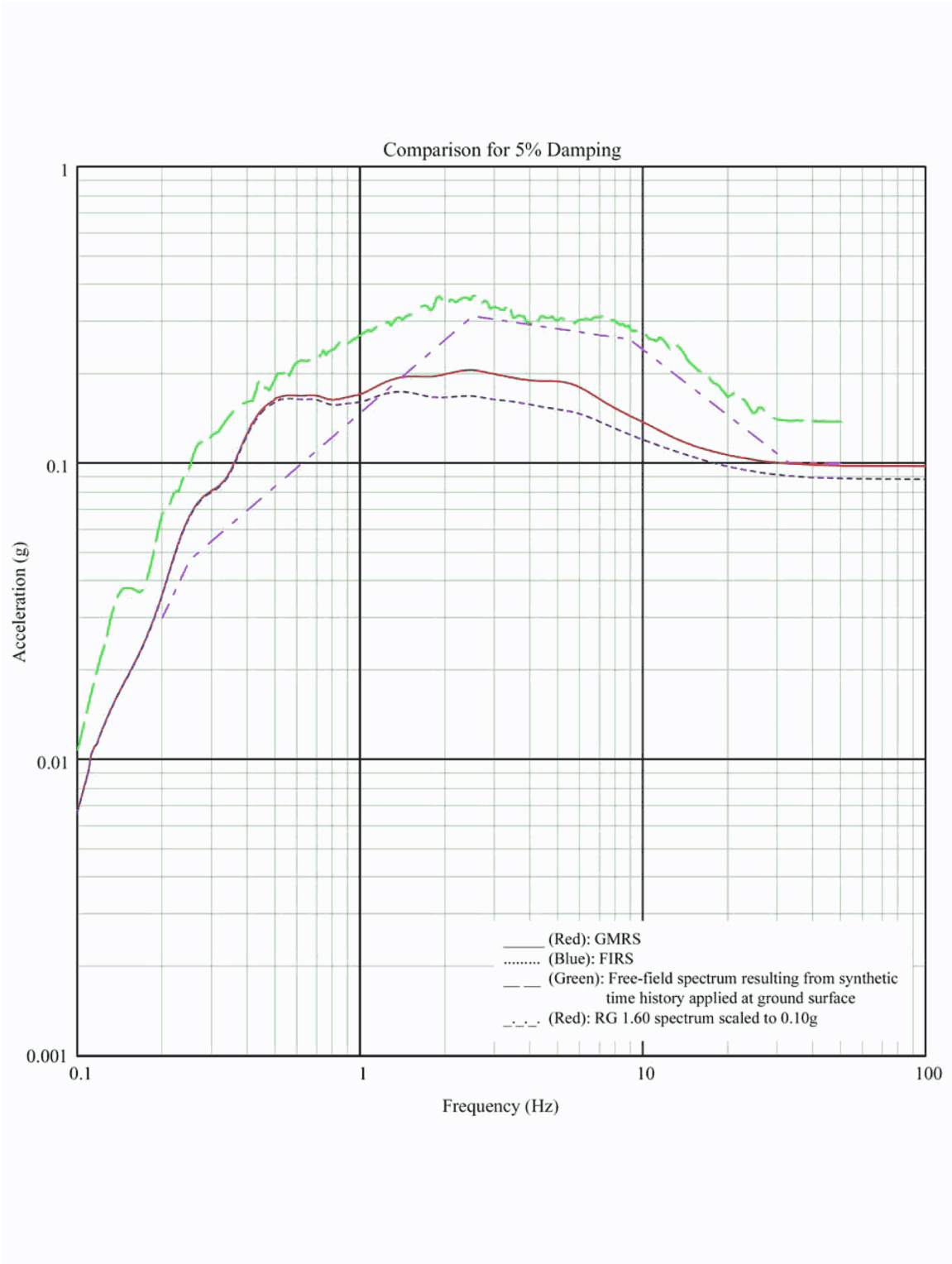
Figure 3A-245 Comparison of Spectra at Foundation of Control Building - Upper Bound Soil Properties, X Direction
