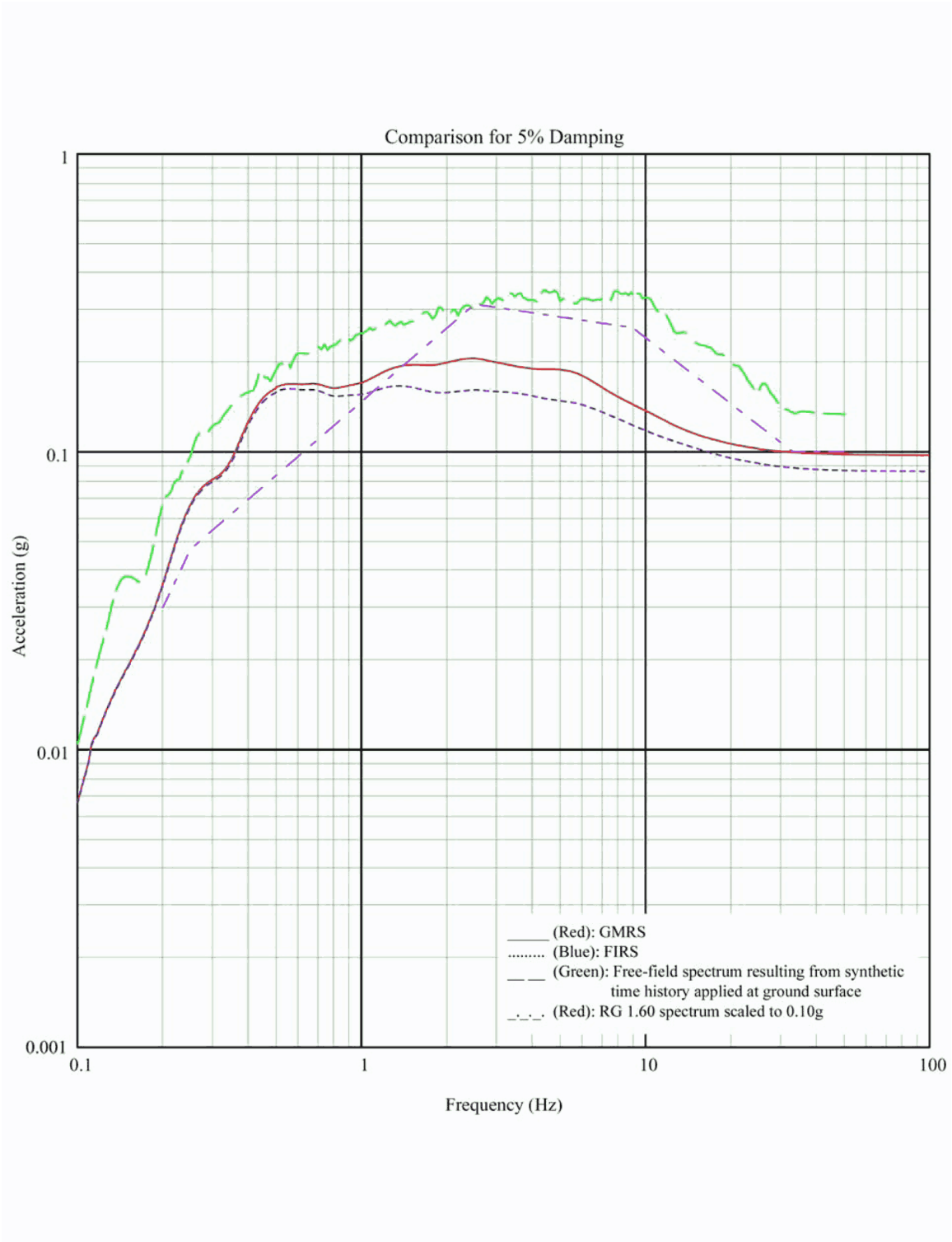
Figure 3A-239 Comparison of Spectra at Foundation of Reactor Building - Lower Bound Soil Properties, X Direction
