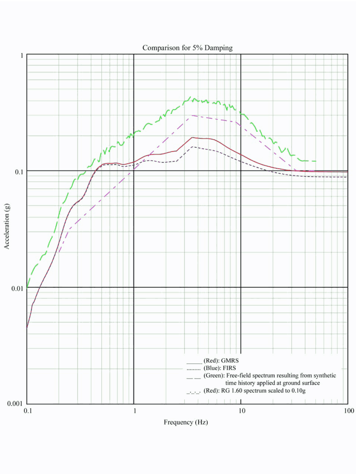
Figure 3A-247 Comparison of Spectra at Foundation of Control Building - Upper Bound Soil Properties, Vertical Direction
