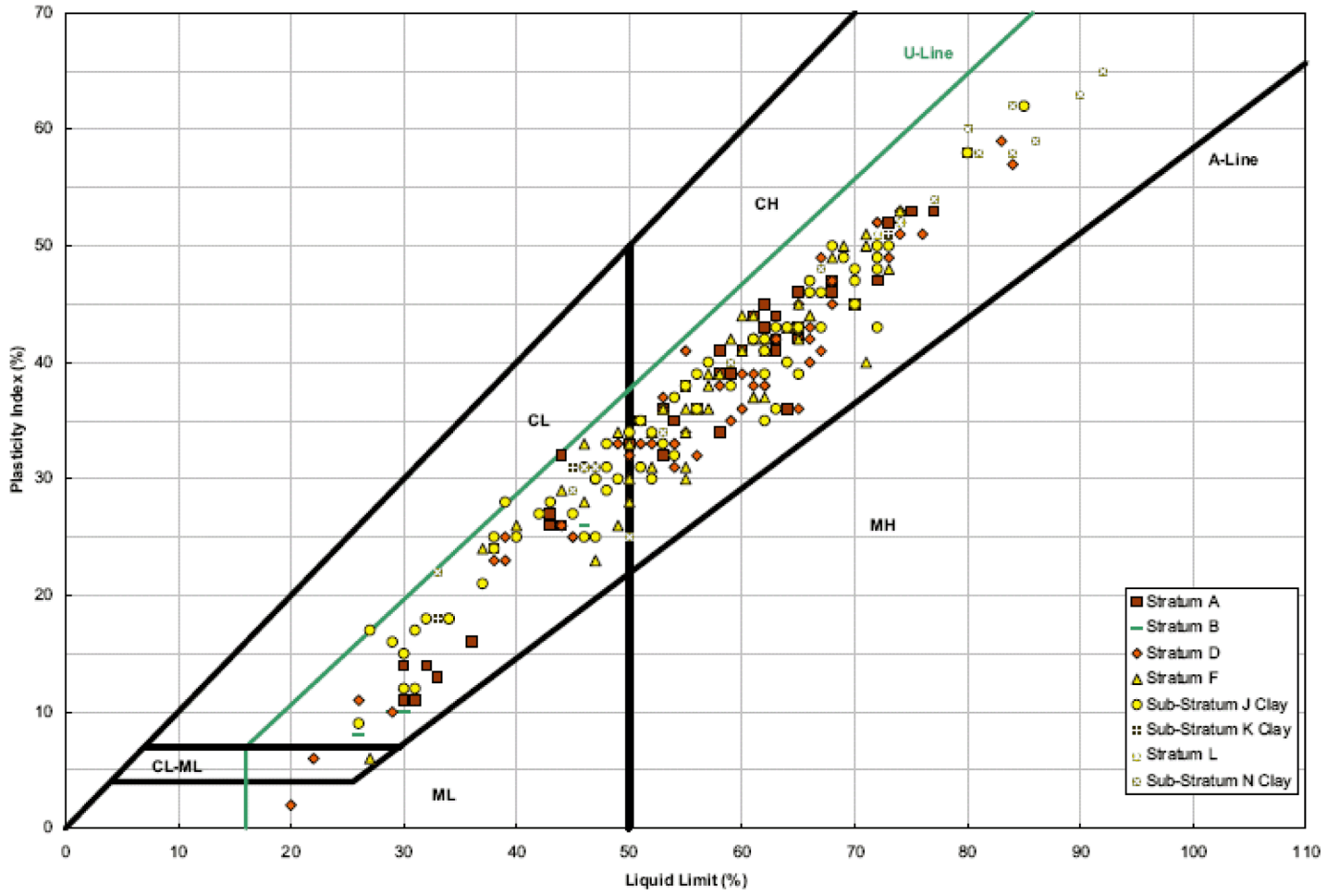
Figure 2.5S.4-21 Plasticity Chart
