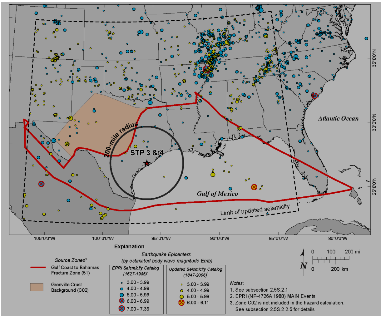
Figure 2.5S.2-4 Rondout Associates EPR1 Source Zones
