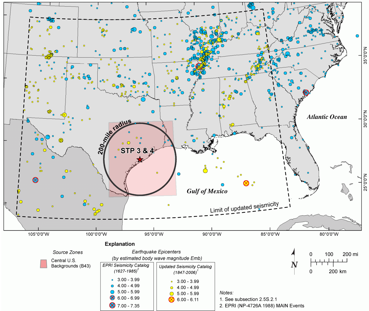
Figure 2.5S.2-6 Woodward-Clyde Consultants EPRi Source Zones
