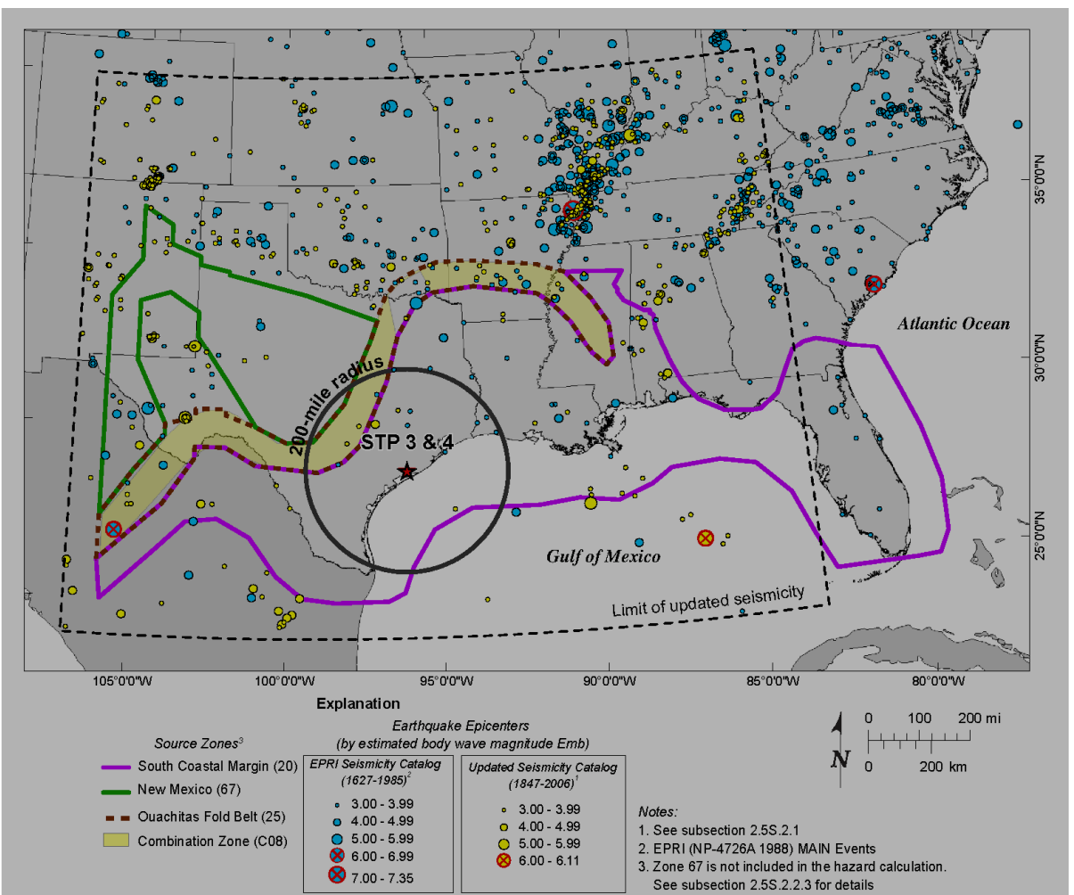
Figure 2.5S.2-2 Dames and Moore EPRI Source Zones
