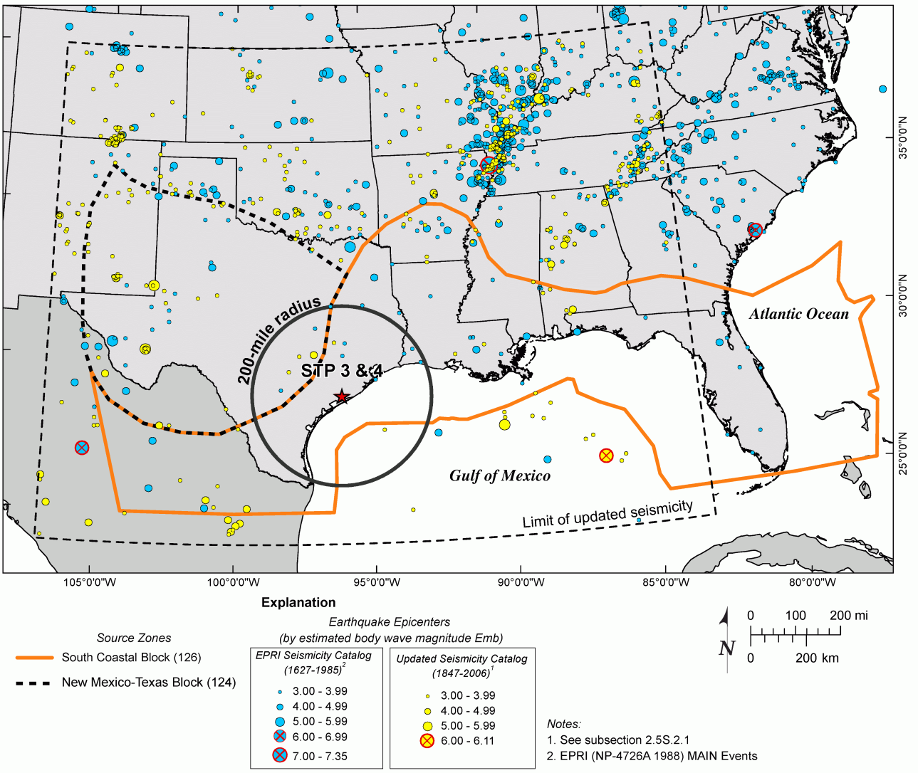
Figure 2.5S.2-3 Law Engineering EPRI (1988) Source Zones
