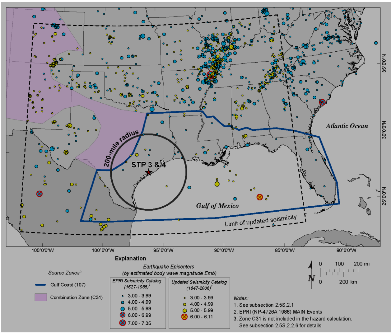
Figure 2.5S.2-5 Weston Geophysical Corporation EPR1 (1989) Source Zones
