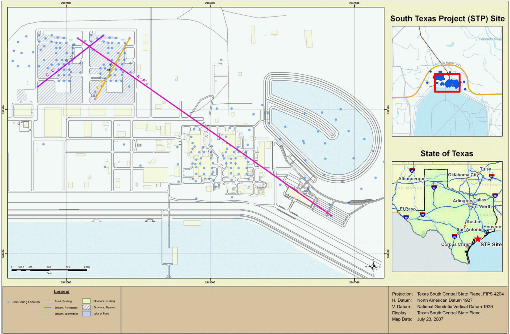
Figure 2.5S.1-31 STP 3 & 4 Cross Section Locations
