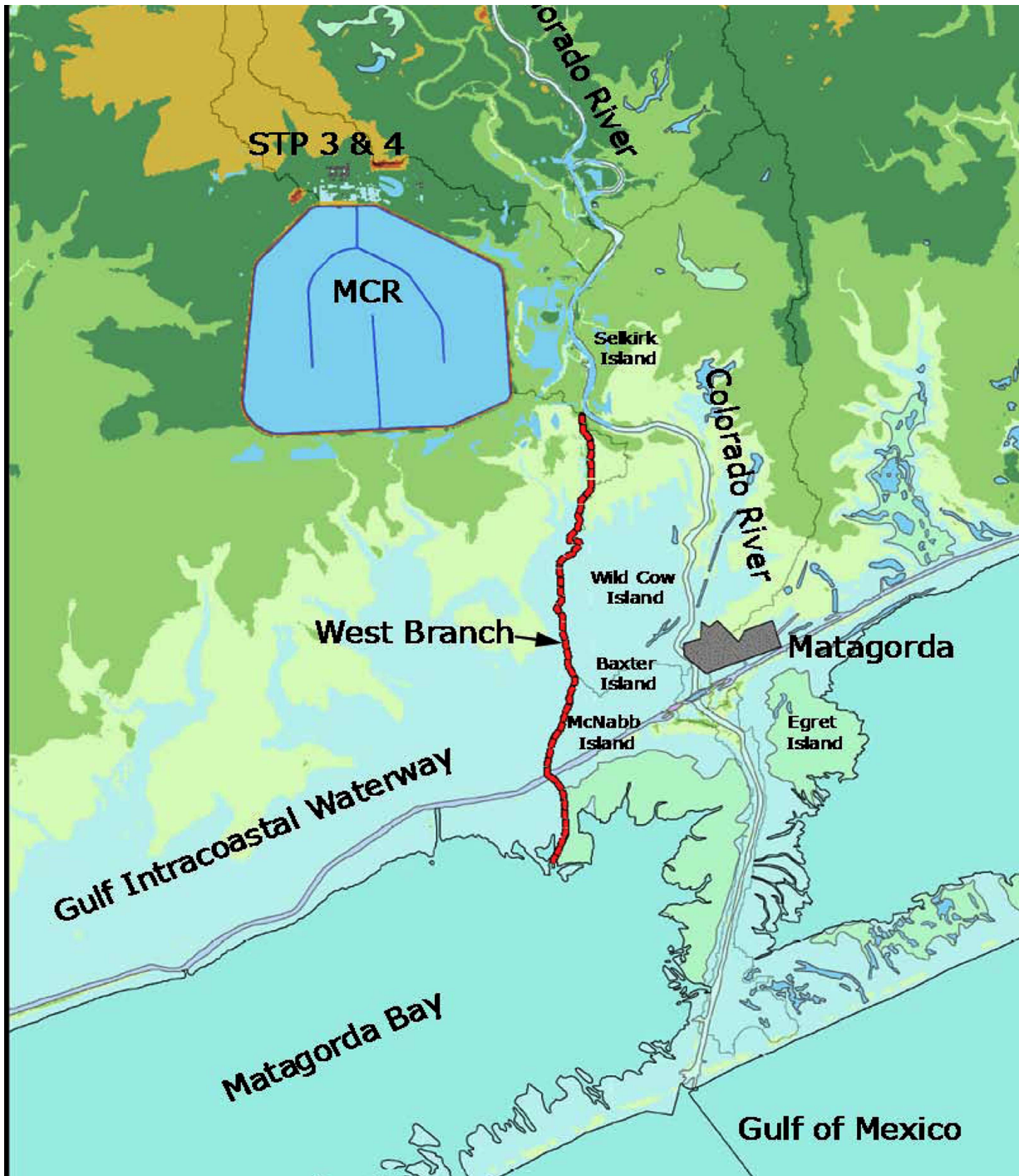
Figure 2.4S.9-9 Plan View of West Branch of the Lower Colorado River, Wild Cow Island, Baxter Island, and McNabb Island Near Matagorda, Texas
