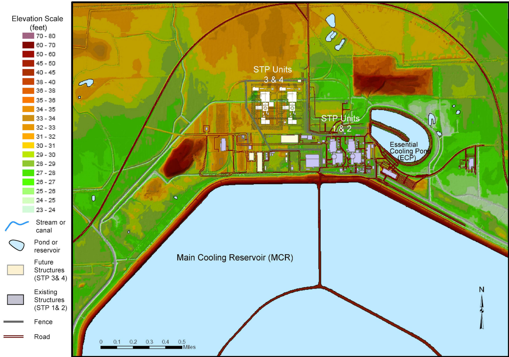
Figure 2.4S.1-3 Existing (Pre-Development) Topography and Major Structures at STP 3 & 4
