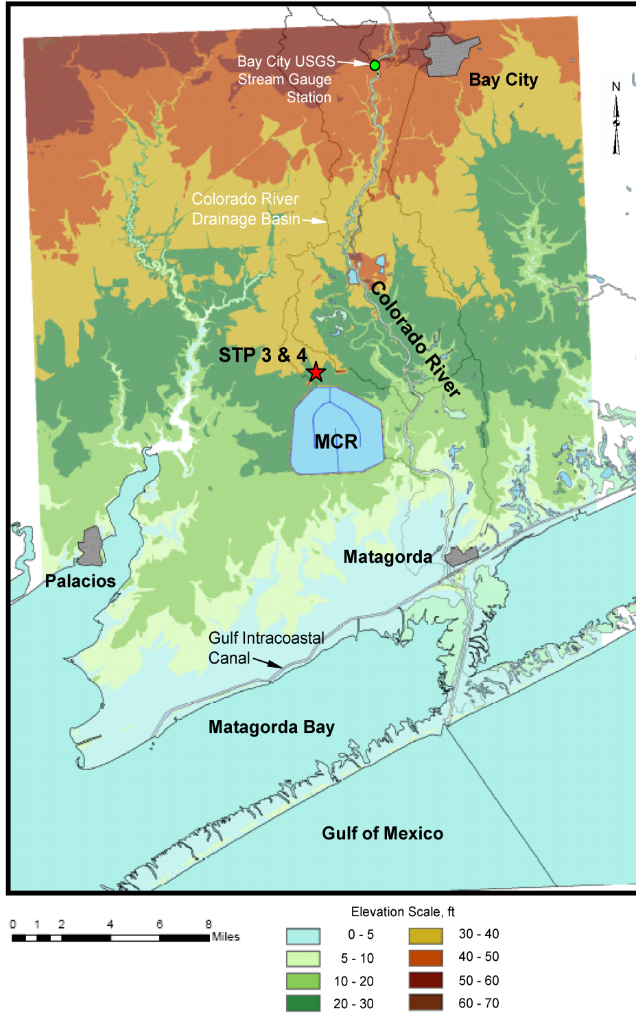
Figure 2.4S.1-1 Site Map of the General Area of STP 3 & 4
