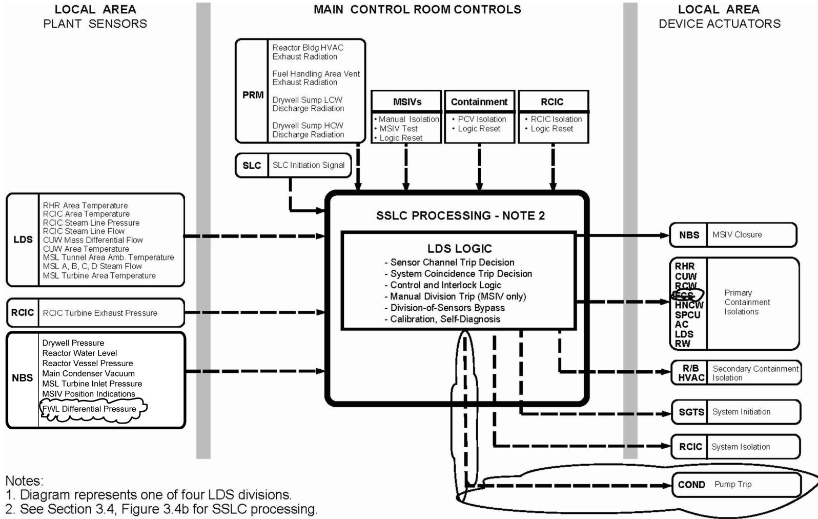
Figure 2.4.2 Leak Detection and Isolation System Interface Diagram
