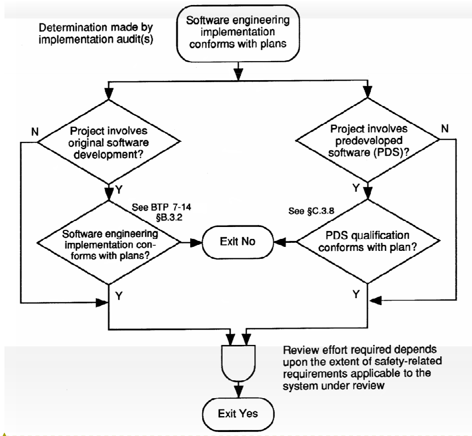
Figure 7.0-A-8. Review of software development process implementation.
