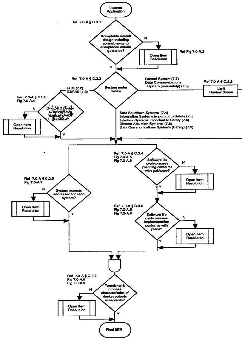
Figure 7.0 A 1. Overview of the process for reviewing digital
