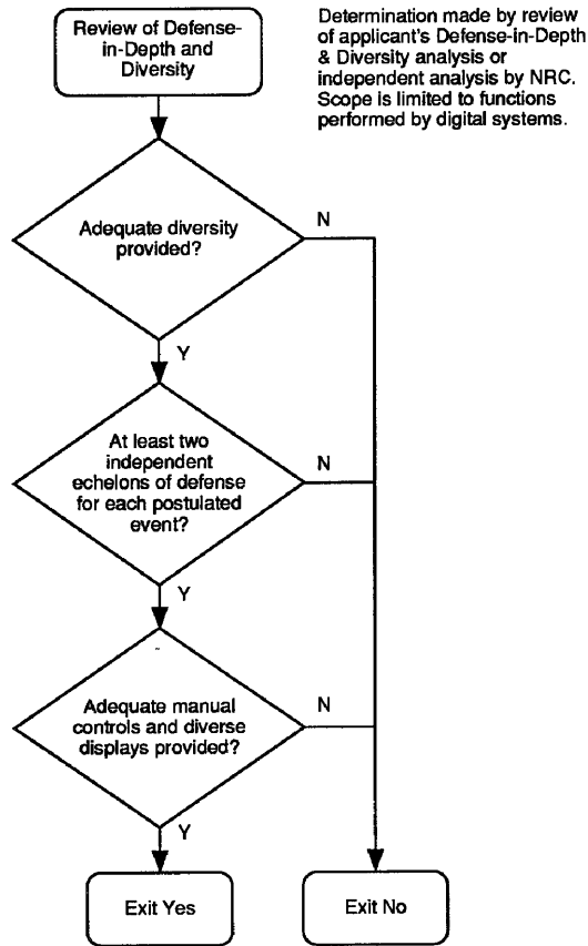
Figure 7.0-A-4. Diversity and Defense-in-Depth review.
