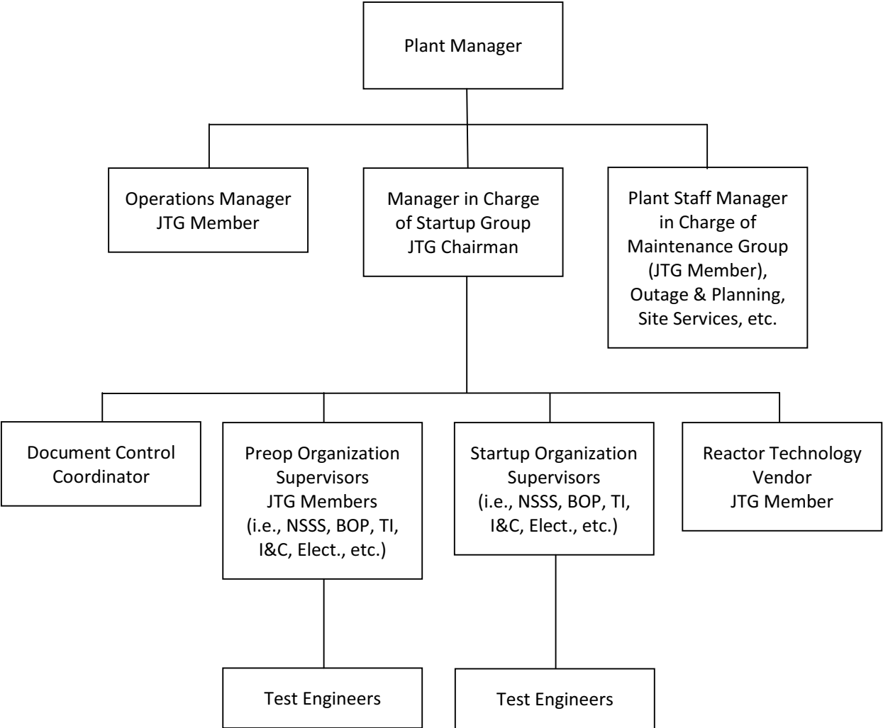
Figure 14AA-201 Preoperational and Startup Test Organization (Typical)
