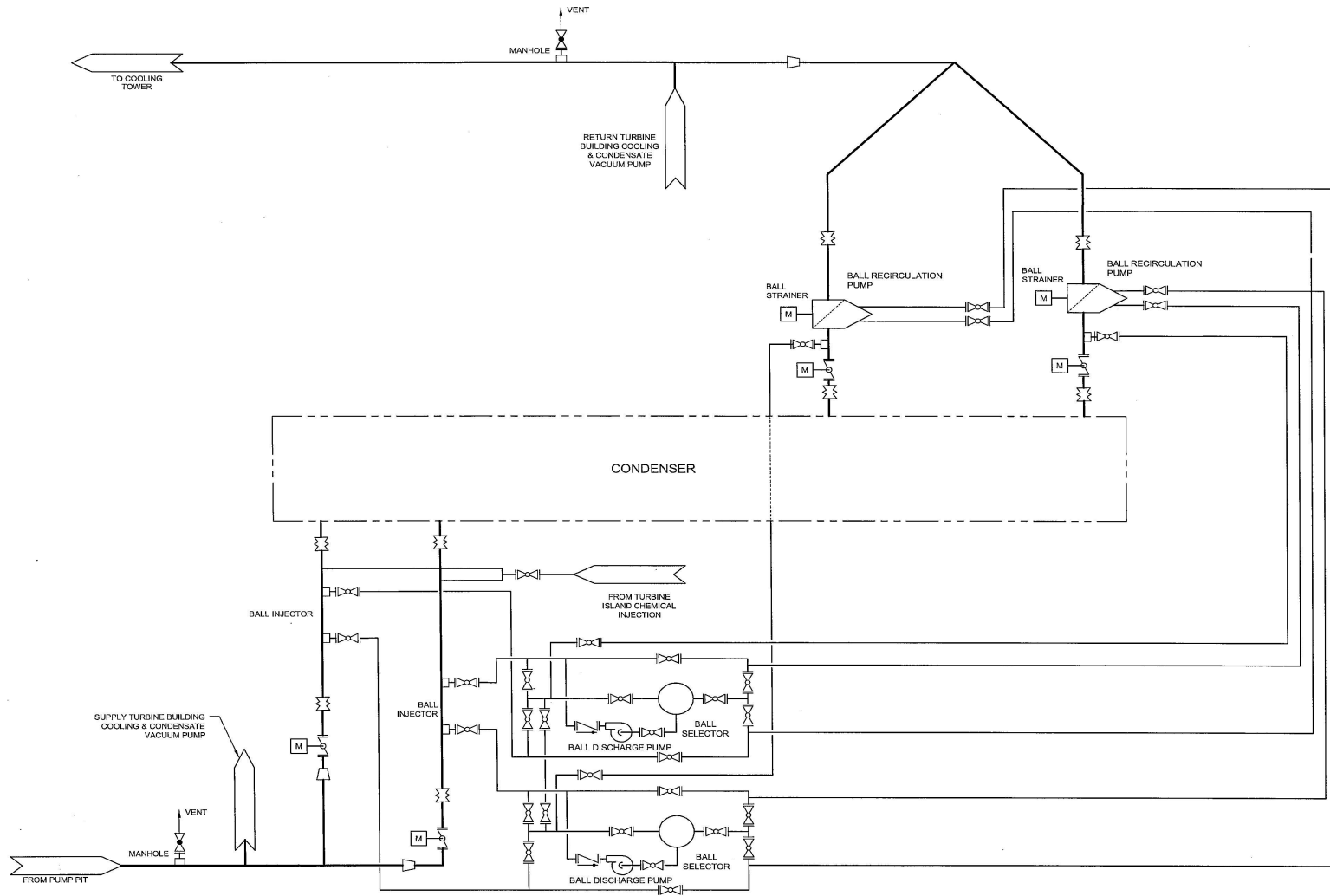
Figure 10.4-202 Condenser and Ball Cleaning System
