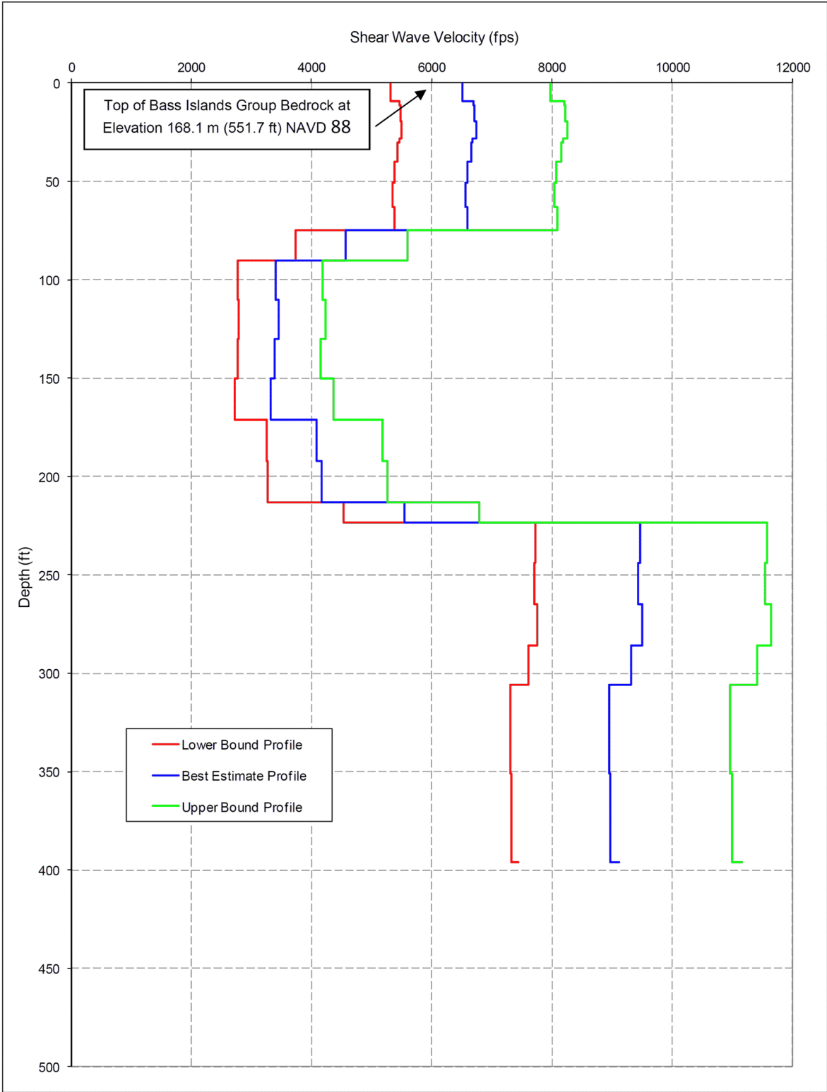
Figure 3.7.1-223 Deterministic Shear Wave Velocity Profiles for the Soil Column without Engineered Granular Backfill Above the Top of the Bass Islands Group Bedrock [EF3 SUP 3.7-1]
