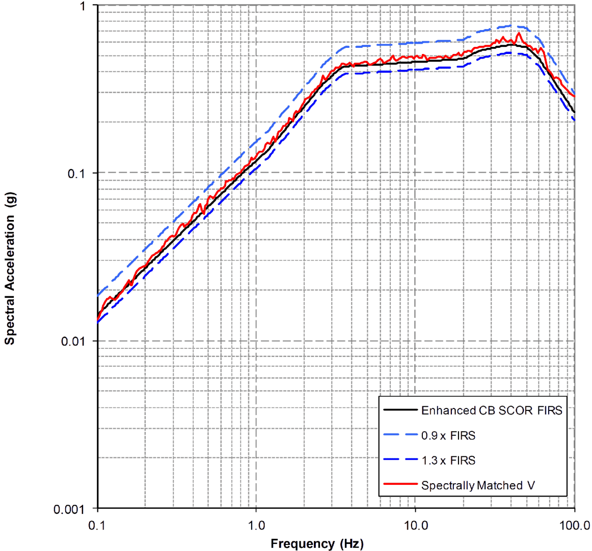
Figure 3.7.1-244 Response Spectrum for Spectrally Matched Vertical (V) Component for the Fermi 3 CB Enhanced SCOR FIRS [EF3 SUP 3.7-1]
