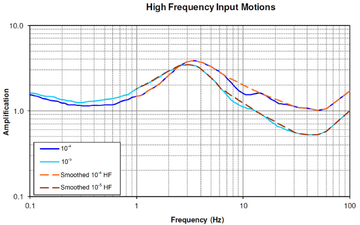
Figure 3.7.1-211 PBSRS Amplification Functions for the Fermi 3 Site [EF3 SUP 3.7-1]
