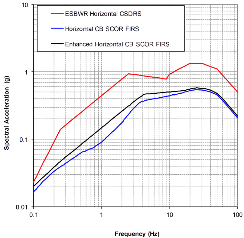
Figure 3.7.1-229 Fermi 3 Horizontal CB SCOR FIRS and Enhanced CB SCOR FIRS (5 Percent Damping) [EF3 COL 2.0-27-A, EF3 SUP 3.7-1]
