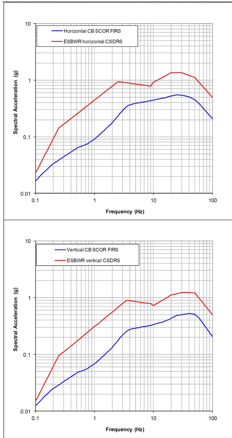
Figure 3.7.1-225 Fermi 3 CB SCOR FIRS (5 Percent Damping) [EF3 COL 2.0-27-A, EF3 SUP 3.7-1]
