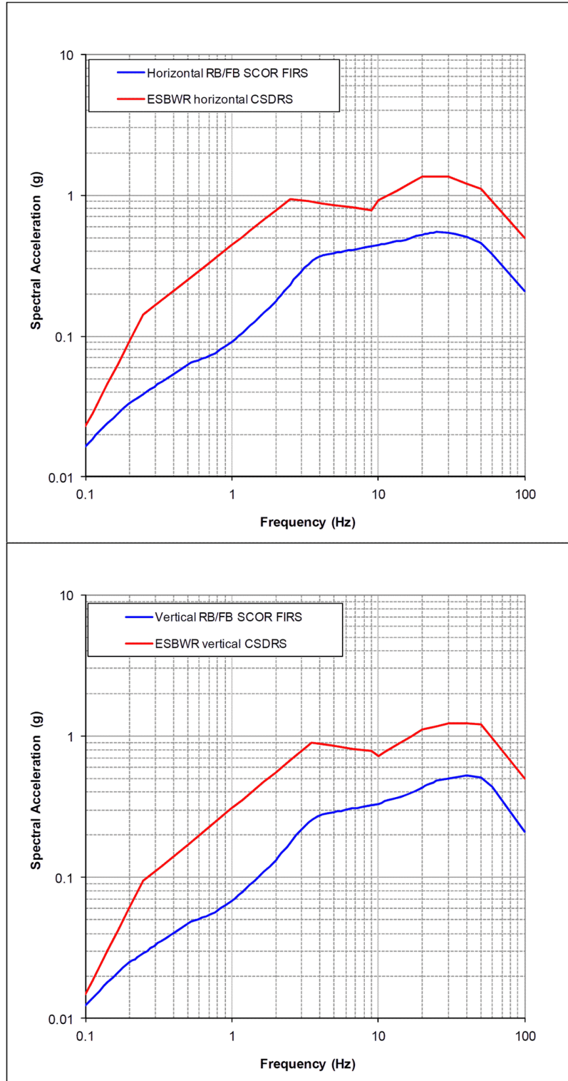
Figure 3.7.1-224 Fermi 3 RB/FB SCOR FIRS (5 Percent Damping) [EF3 COL 2.0-27-A, EF3 SUP 3.7-1]
