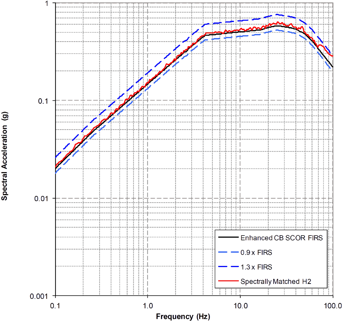
Figure 3.7.1-243 Response Spectrum for Spectrally Matched Horizontal (H2) Component for the Fermi 3 CB Enhanced SCOR FIRS [EF3 SUP 3.7-1]
