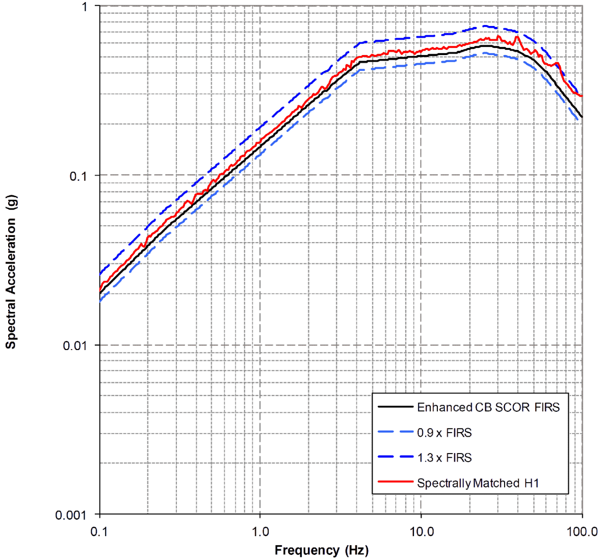
Figure 3.7.1-242 Response Spectrum for Spectrally Matched Horizontal (H1) Component for the Fermi 3 CB Enhanced SCOR FIRS [EF3 SUP 3.7-1]
