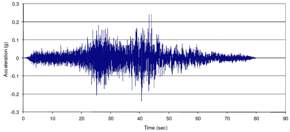
Figure 3.7.1-248 Acceleration, Velocity, and Displacement Time Histories for the Spectrally Matched Horizontal (H1) Component Compatible with the Fermi 3 CB Enhanced SCOR FIRS [EF3 SUP 3.7-1]
