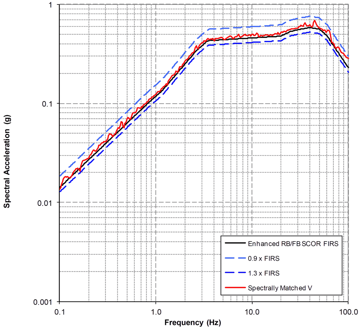
Figure 3.7.1-241 Response Spectrum for Spectrally Matched Vertical (V) Component for the Fermi 3 RB/FB Enhanced SCOR FIRS [EF3 SUP 3.7-1]
