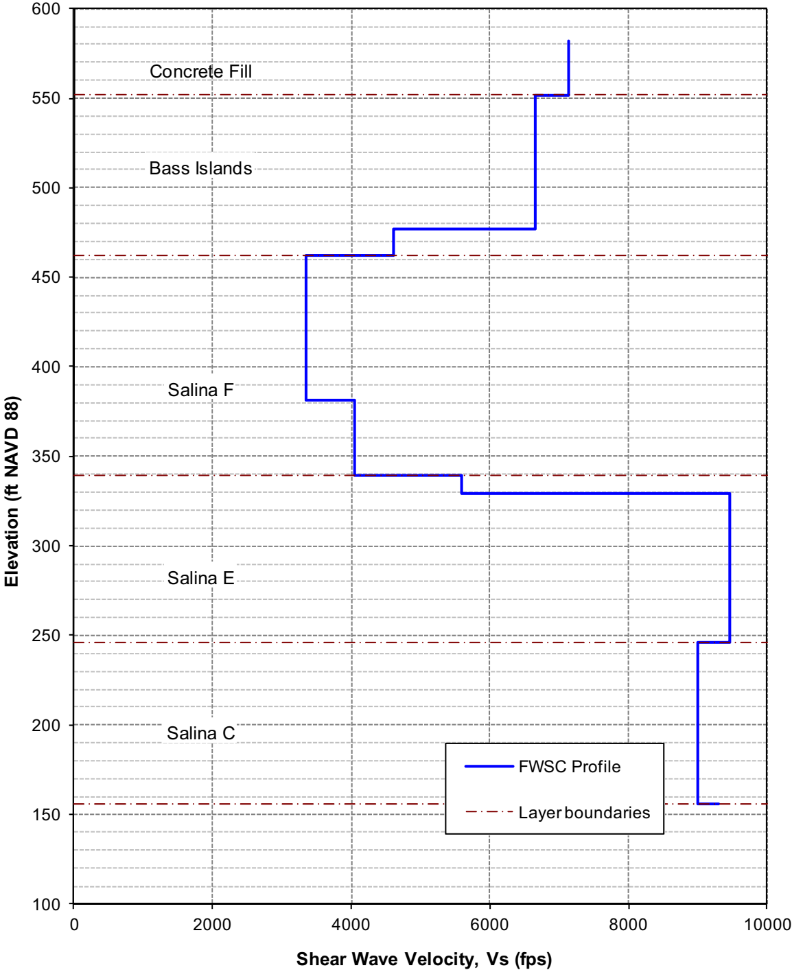
Figure 3.7.1-202 Shear Wave Velocity Profiles for Site Response Analysis: FWSC Shear Wave Velocity Profile [EF3 COL 2.0-27-A, EF3 SUP 3.7-1]
