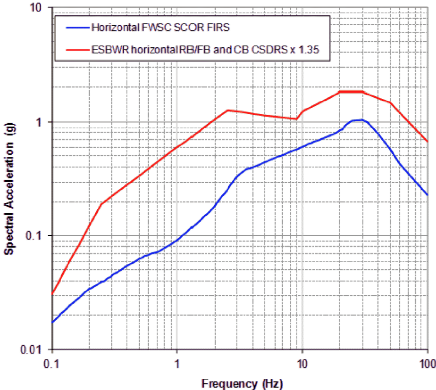
Figure 3.7.1-238 Fermi 3 FWSC FIRS (5 Percent Damping) [EF3 COL 2.0-27-A, EF3 SUP 3.7-1]
