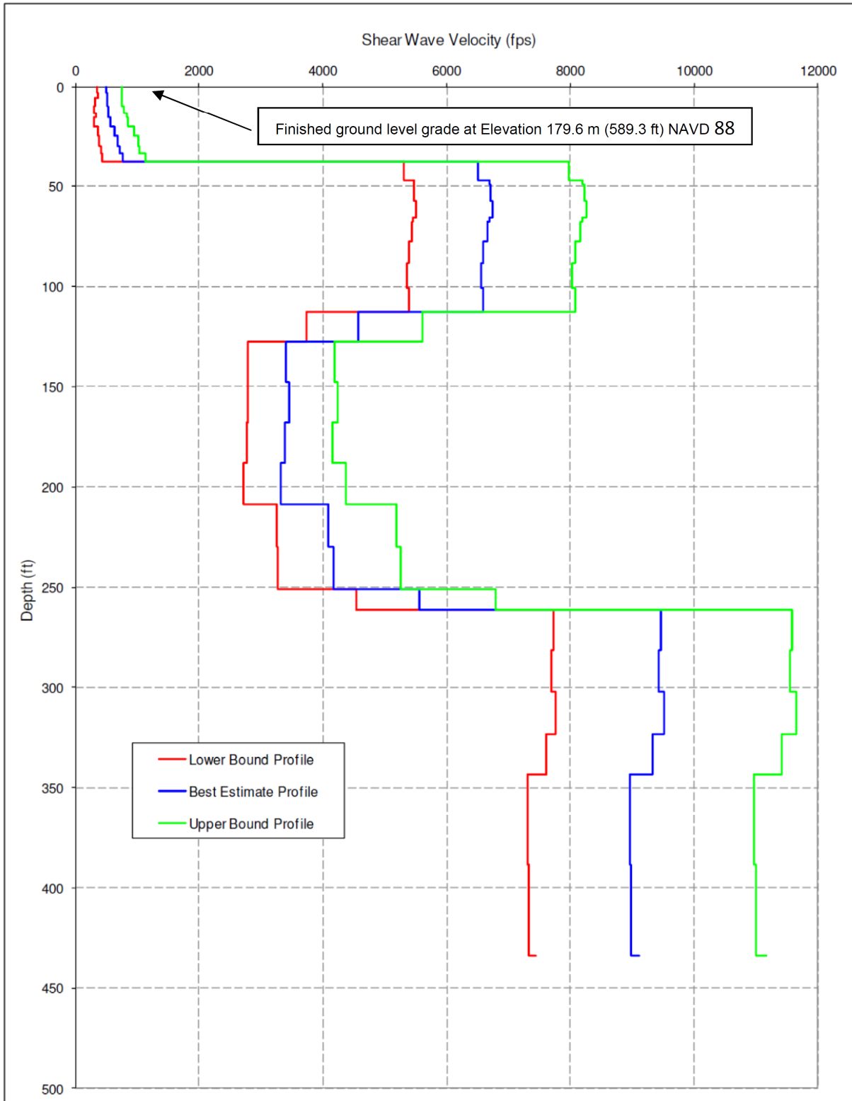
Figure 3.7.1-222 Deterministic Shear Wave Velocity Profiles for the Full Soil Column with Engineered Granular Backfill Above the Top of the Bass Islands Group Bedrock [EF3 SUP 3.7-1]
