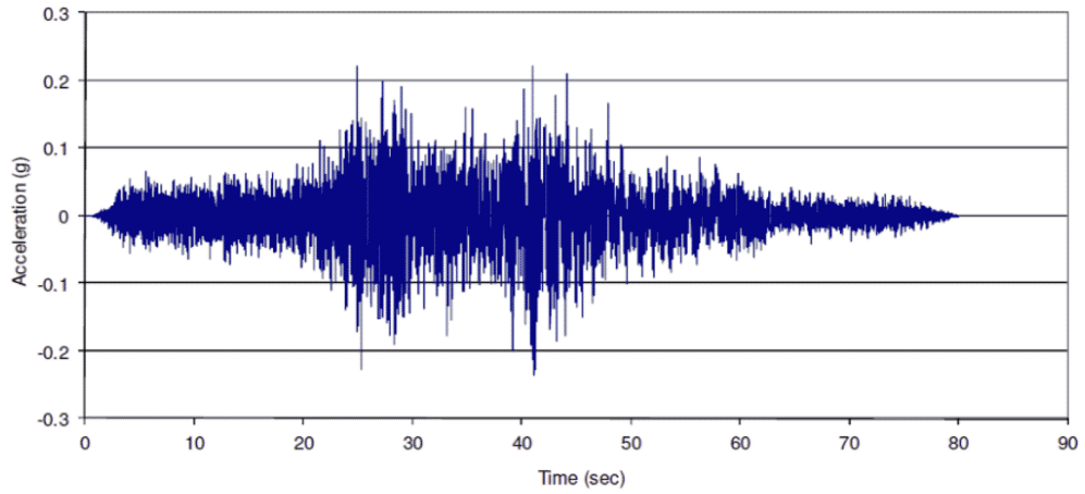
Figure 3.7.1-246 Acceleration, Velocity, and Displacement Time Histories for the Spectrally Matched Horizontal (H2) Component Compatible with the Fermi 3 RB/FB Enhanced SCOR FIRS [EF3 SUP 3.7-1]
