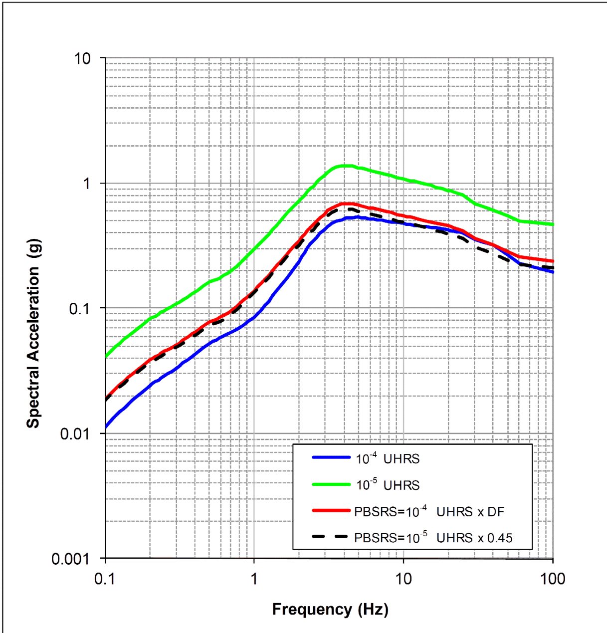
Figure 3.7.1-219 Development of the Horizontal PBSRS for the Fermi 3 Site [EF3 SUP 3.7-1]
