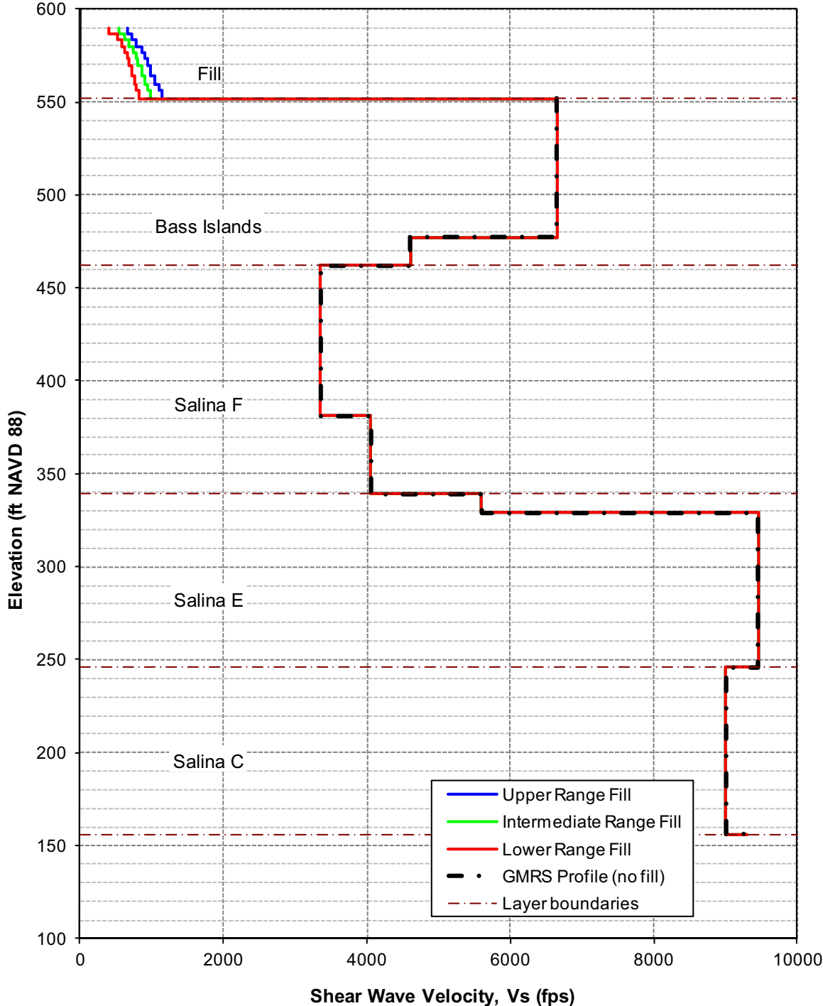
Figure 3.7.1-201 Shear Wave Velocity Profiles for Site Response Analysis: Intermediate Range, Lower Range, and Upper Range Values [EF3 COL 2.0-27-A, EF3 SUP 3.7-1]
