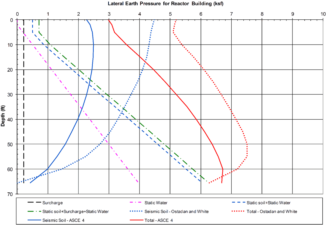
Figure 2.5.4-229 Lateral Earth Pressure on Reactor Building Walls [EF3 COL 2.0-29-A]
