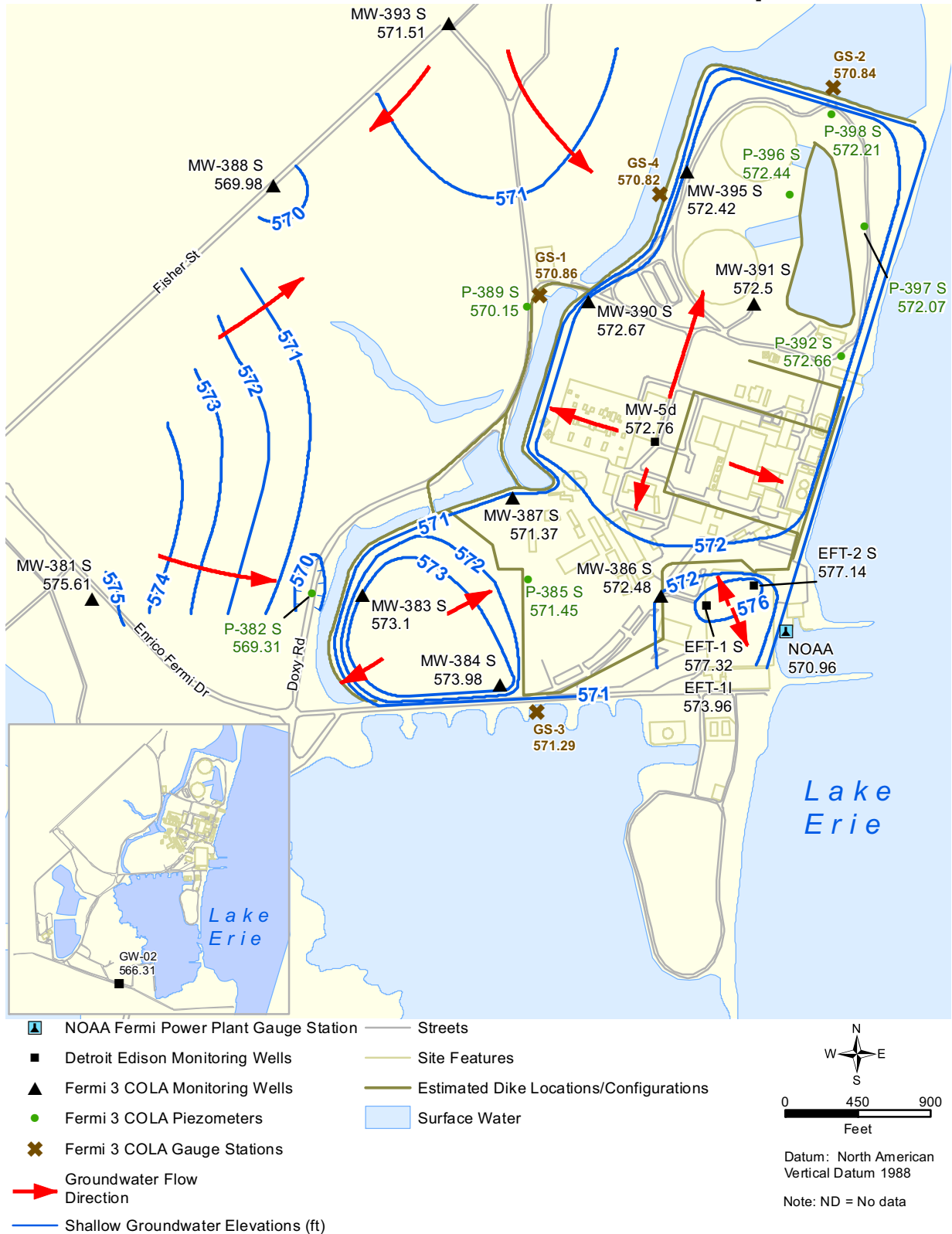
Figure 2.4-243 Overburden Water Table Map 09/28/2007-09/29/2007 [EF3 COL 2.0-23-A]
