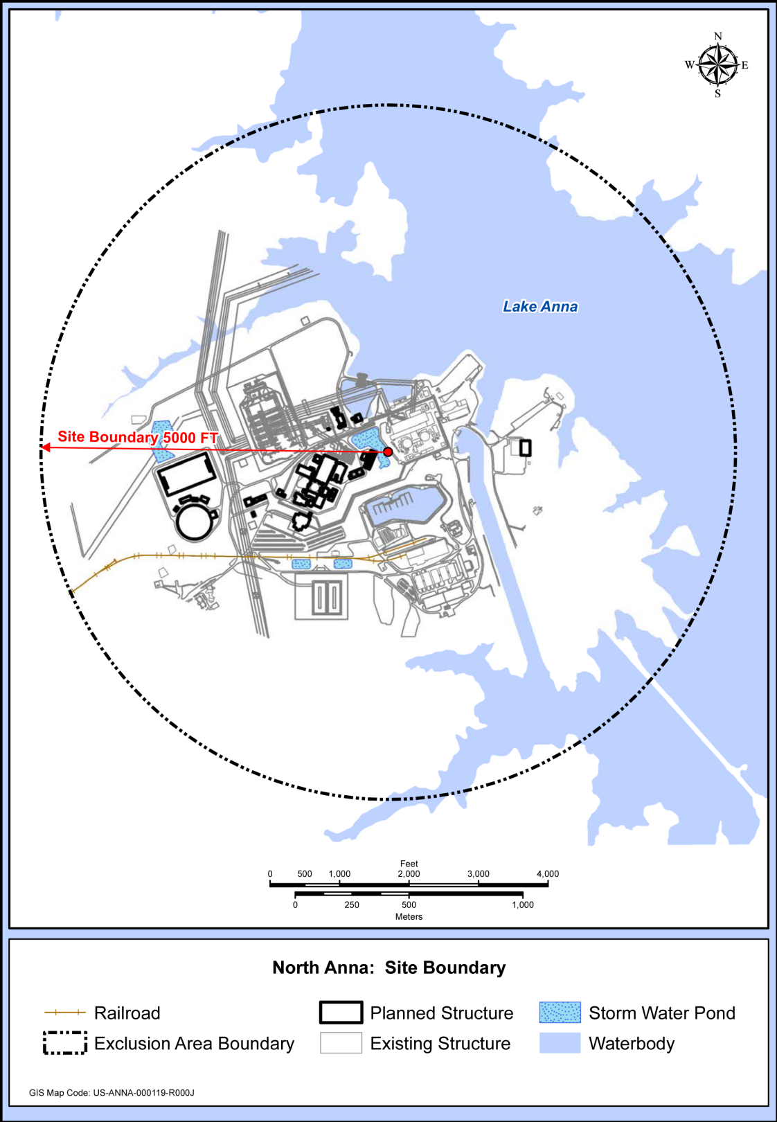
NAPS COL 2.0-3-A Figure 2.1-1R Site Boundary
