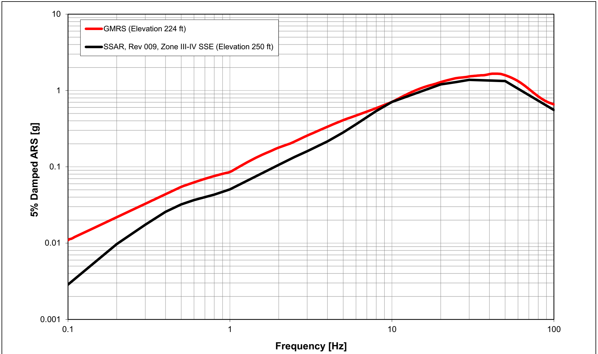
Figure 2.0-207 Comparison of the ESP Vertical SSE Design Response Spectrum for the Top of Zone III-IV and Unit 3 Vertical GMRS
