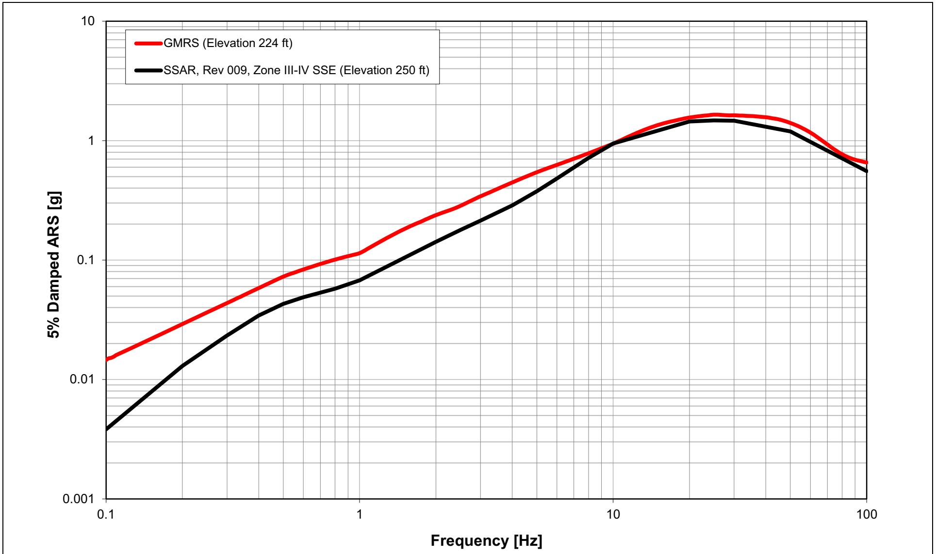
Figure 2.0-206 Comparison of the ESP Horizontal SSE Design Response Spectrum for the Top of Zone III-IV and Unit 3 Horizontal GMRS
