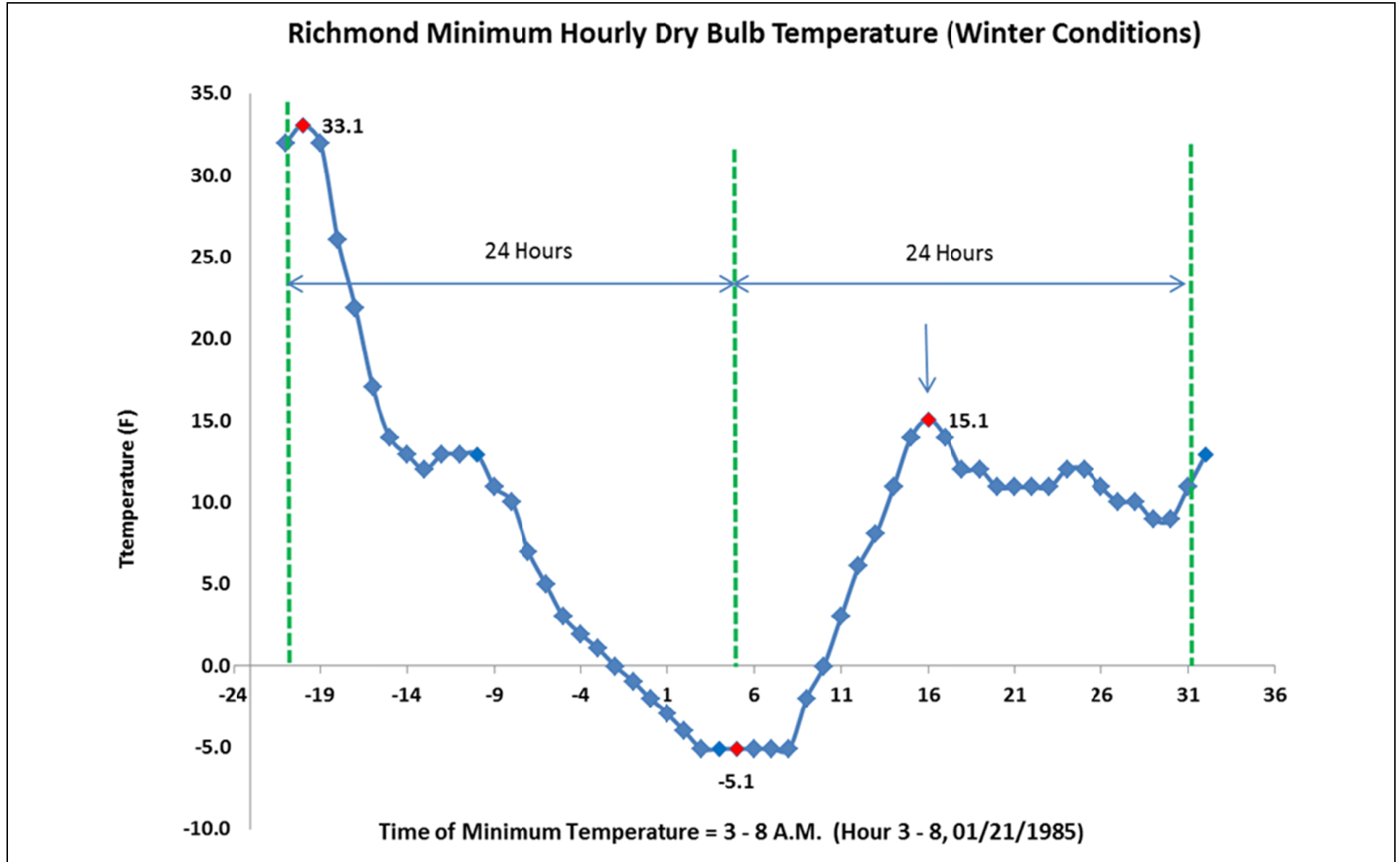
Figure 2.3-203 Hourly Dry Bulb Temperature from Richmond on January 21, 1985
