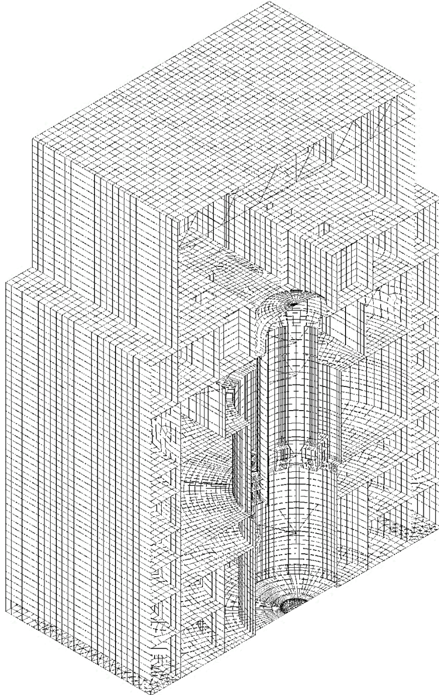
Figure 3F-4. RB/FB 3D Shell Model (90°-270° Direction)
