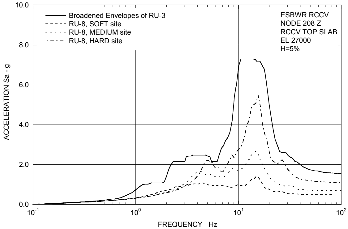
Figure 3A.8.7-3b. FRS (Effect of Embedment) – RCCV Top Slab Z
