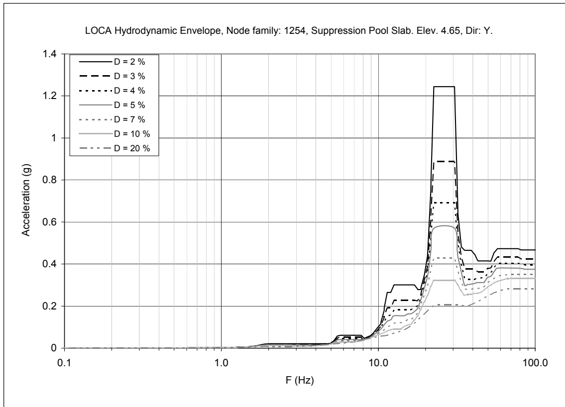
Figure 3F-32. Floor Response Spectra—Chugging & CO Envelope, Node Family: 1254, Y-direction (90°-270°)
