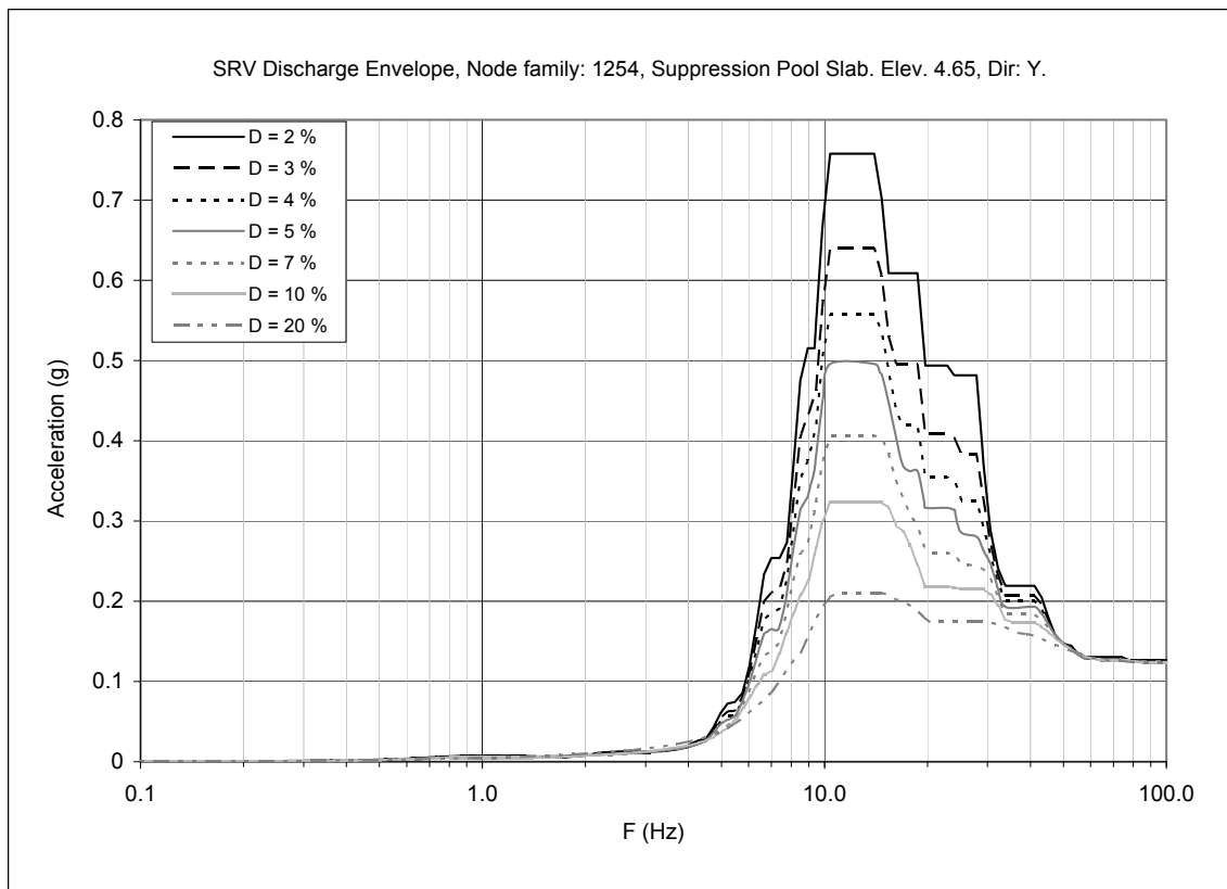
Figure 3F-20. Floor Response Spectra—SRV Discharge Envelope, Node Family: 1254, Y-direction (90°-270°)
