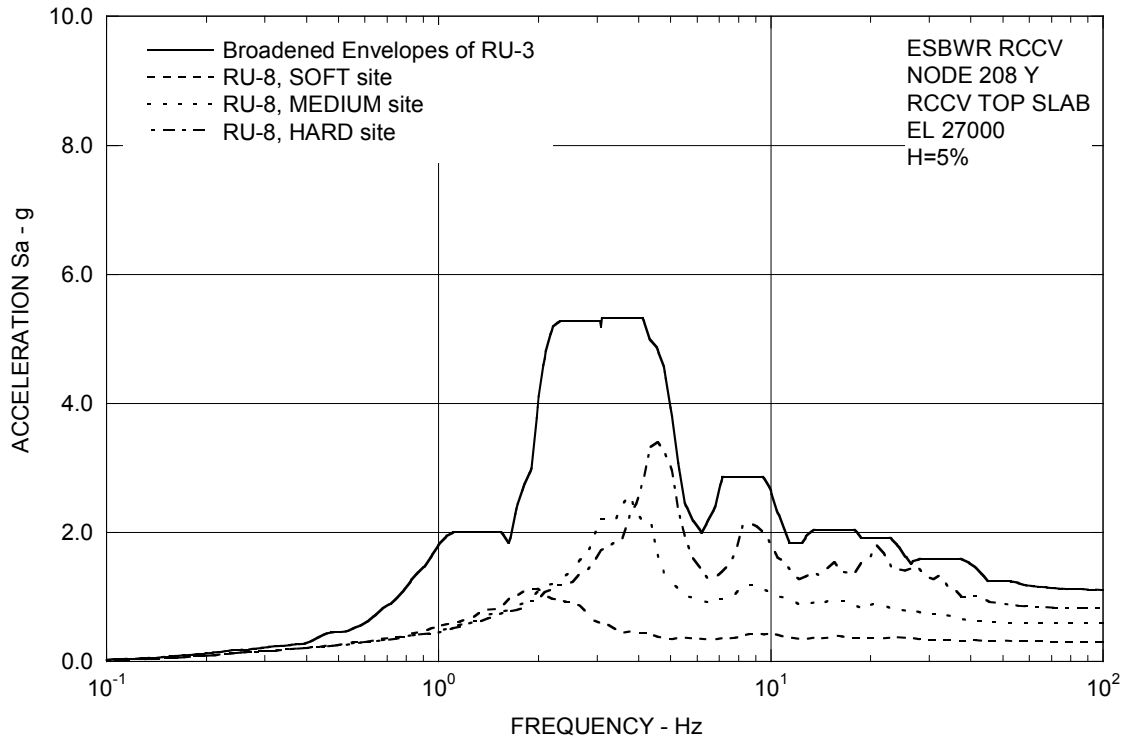
Figure 3A.8.7-2b. FRS (Effect of Embedment) – RCCV Top Slab Y
