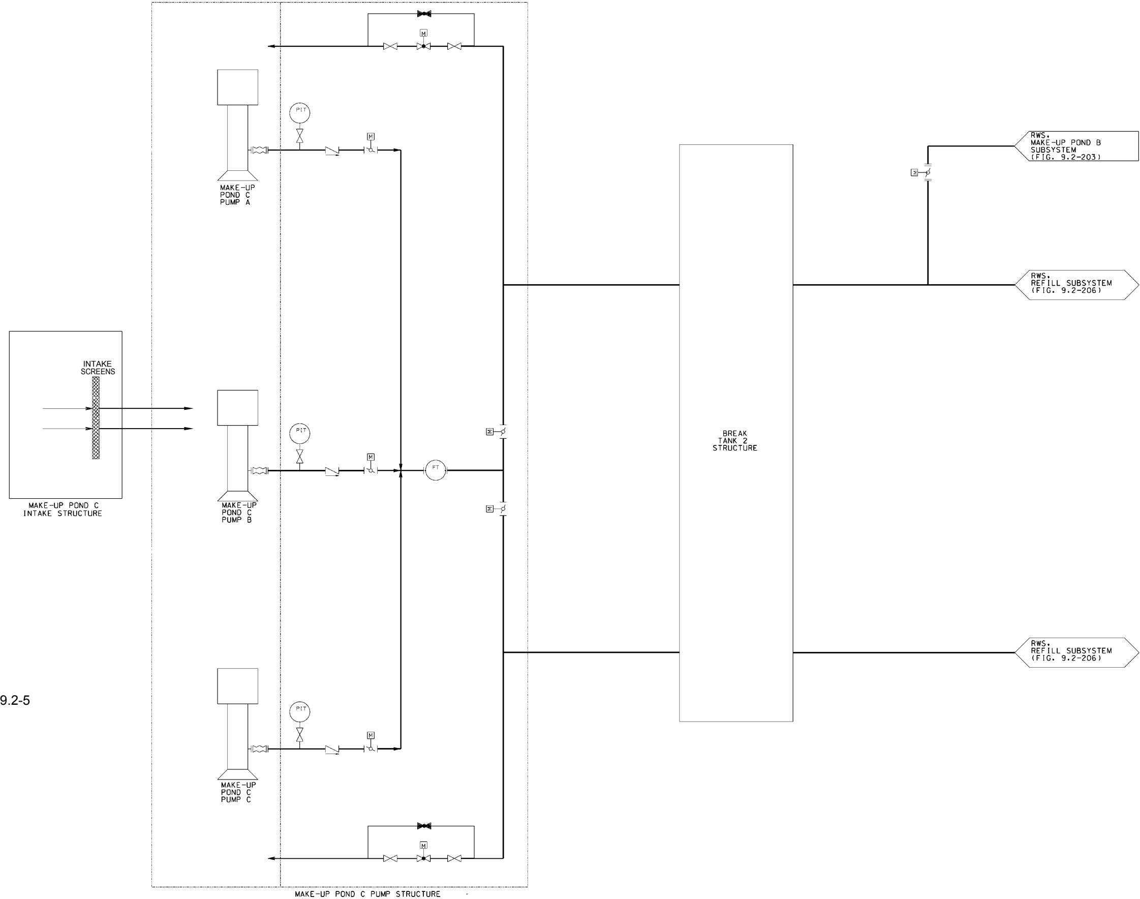
WILLIAM STATES LEE III NUCLEAR STATION UNITS 1 & 2 Raw Water System, Make-Up Pond C Subsystem FIGURE 9.2-207 Rev 3
