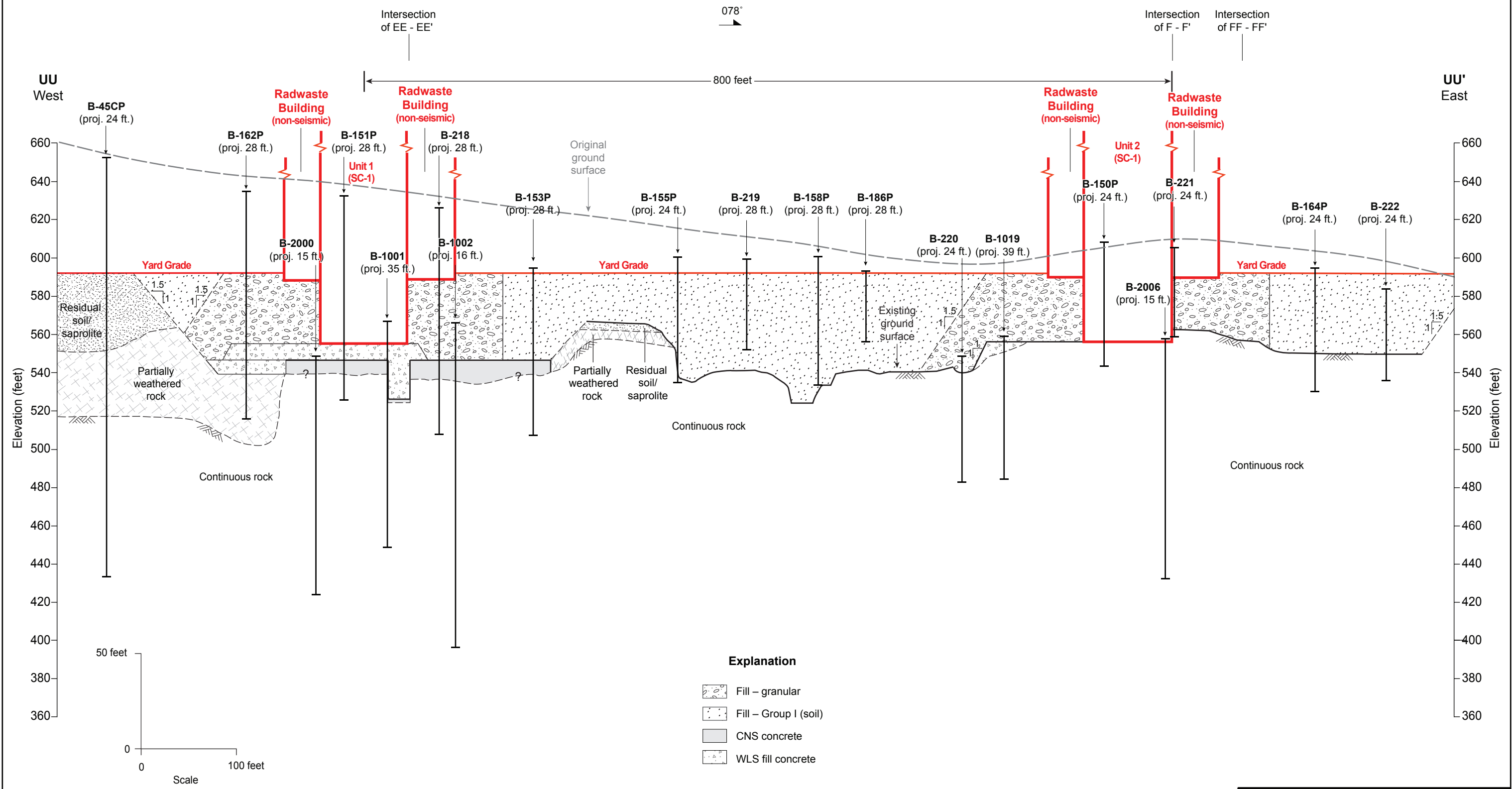
WILLIAM STATES LEE III NUCLEAR STATION UNITS 1 & 2 Planned Excavation Profile, Geologic Cross Section UU-UU' FIGURE 2.5.4-245 Rev 7
