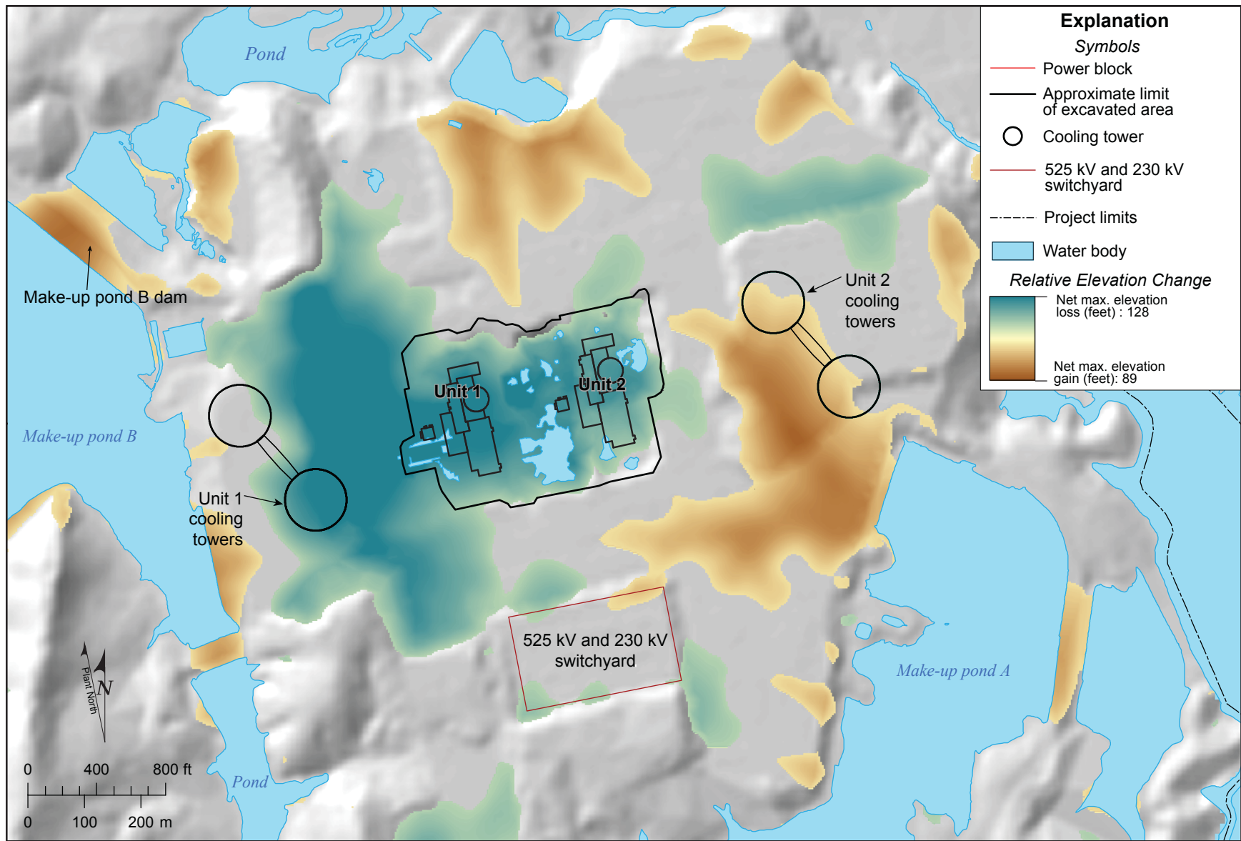
WILLIAM STATES LEE III NUCLEAR STATION UNITS 1 & 2 Topographic Comparison - Representation of Net Topographic Change between 1971 and 2006 FIGURE 2.5.4-202 Rev 7
