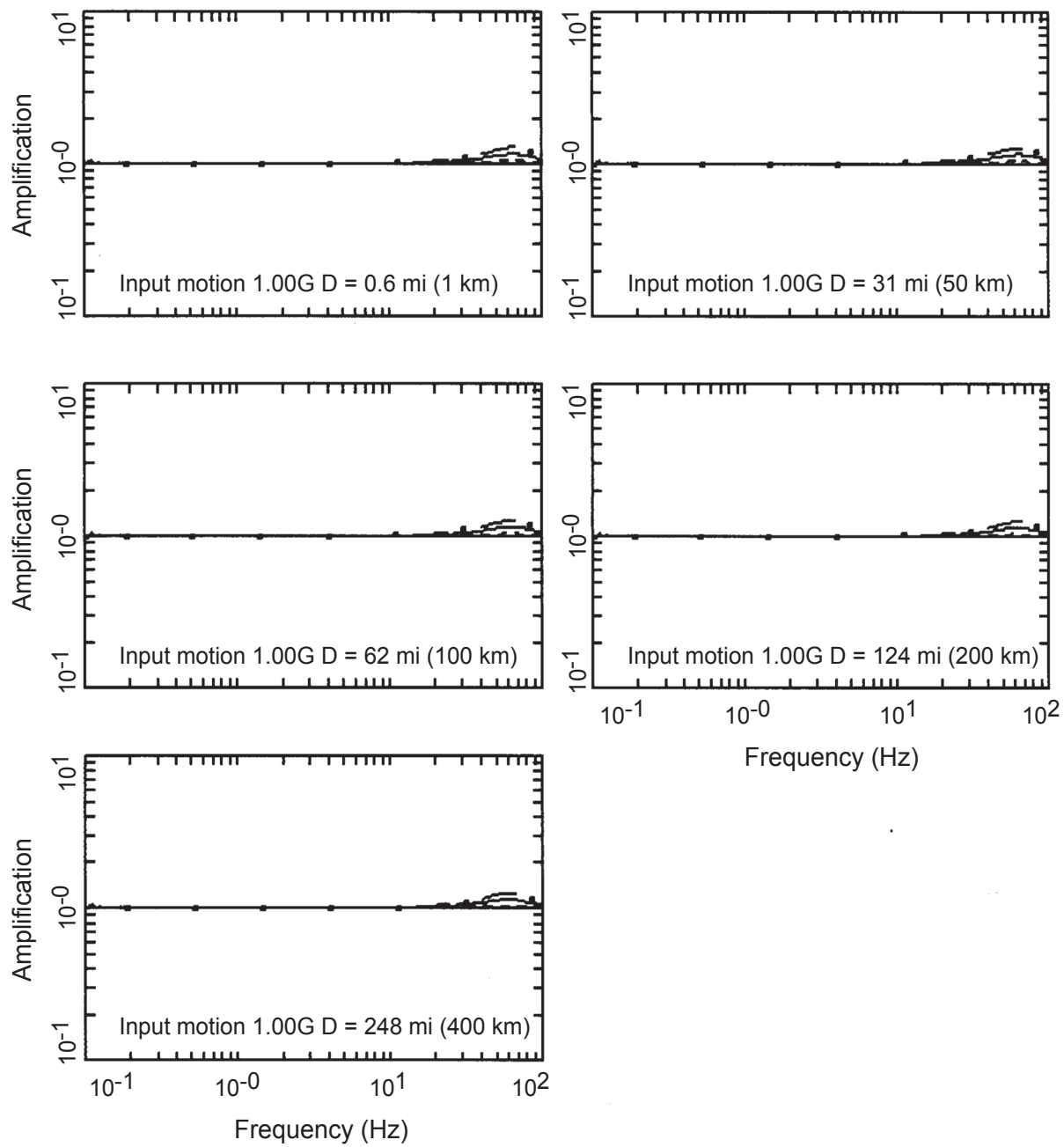
AMPLIFICATION (H), UNIT 1 FIRS A1
