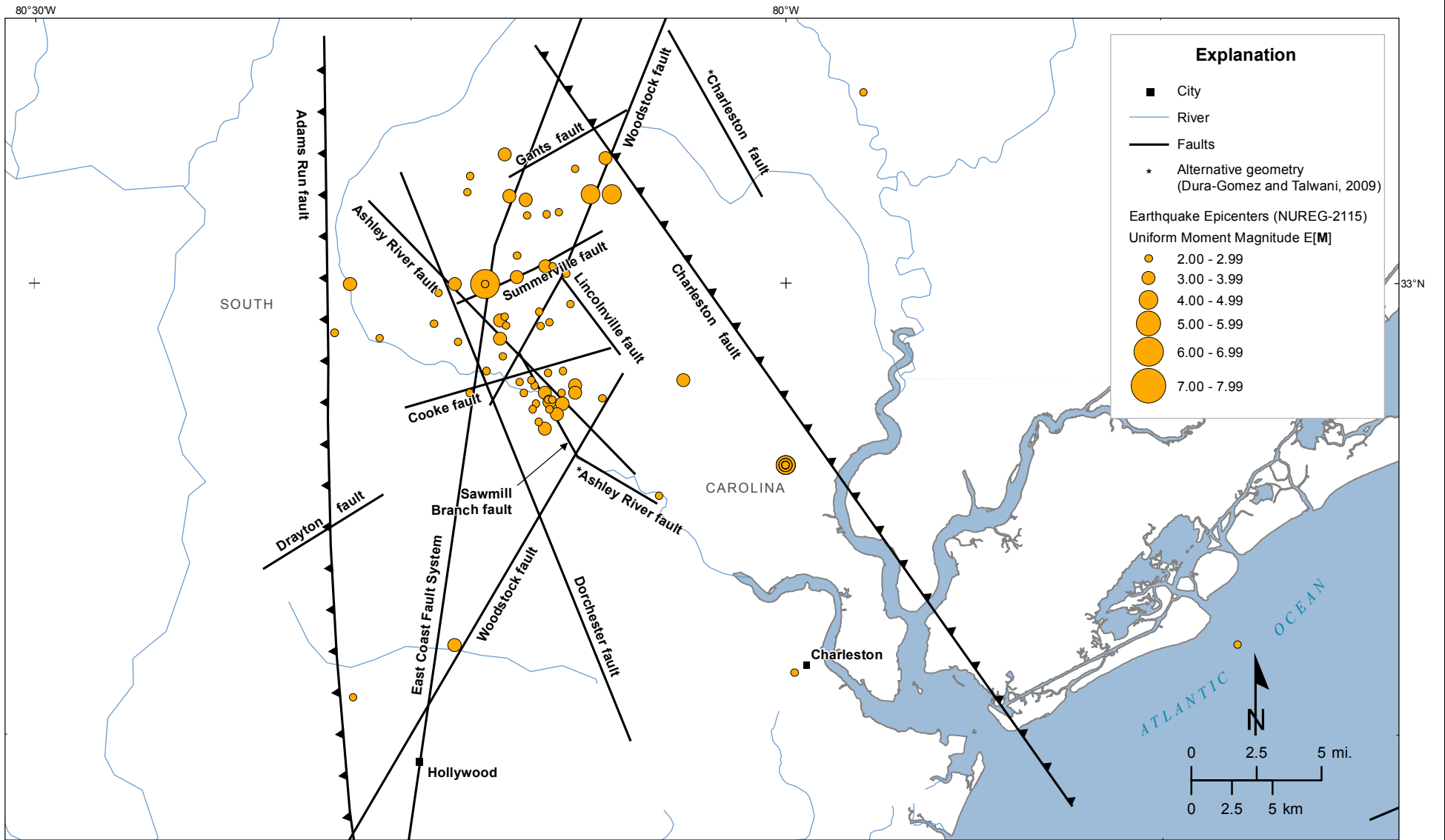
WILLIAM STATES LEE III NUCLEAR STATION UNITS 1 & 2 Charleston Area Seismicity and Postulated Faults FIGURE 2.5.1-217 Rev 8
